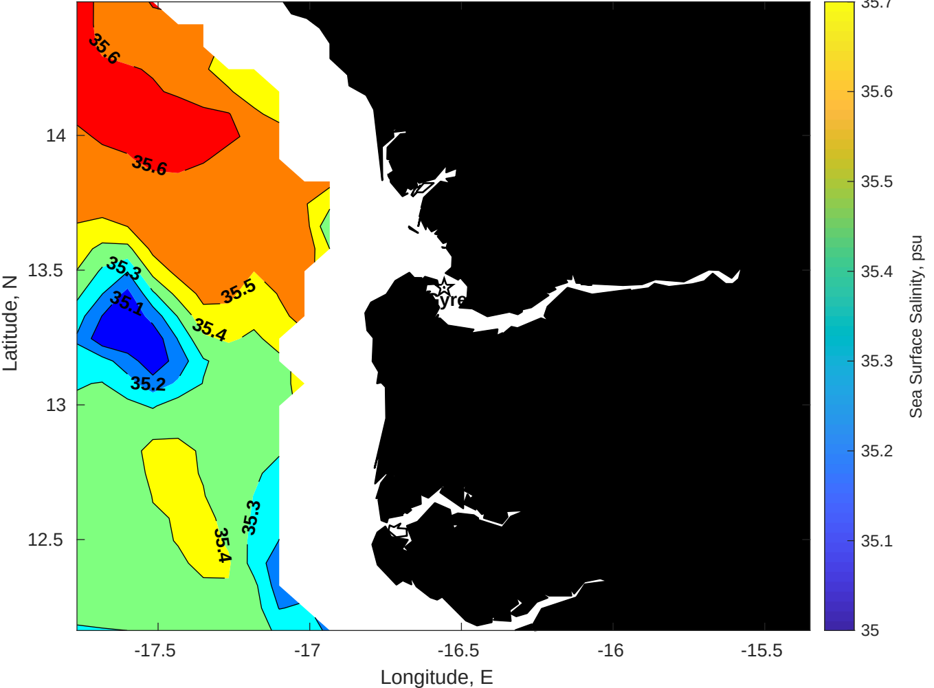
Surface Salinity for Gyre at 07-Aug-2025 00:00:00
