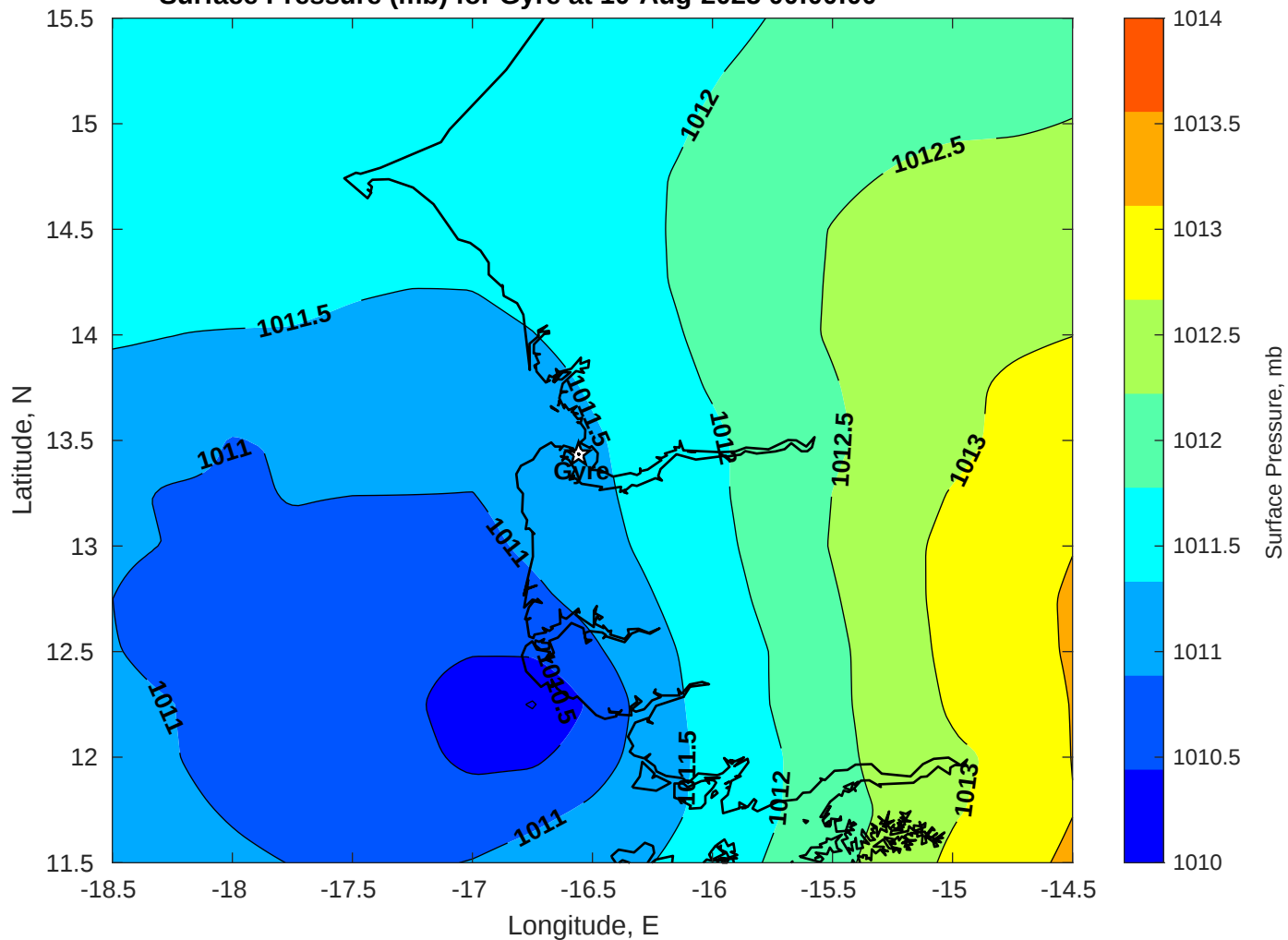
Surface Pressure (mb) for Gyre at 10-Aug-2025 00:00:00
