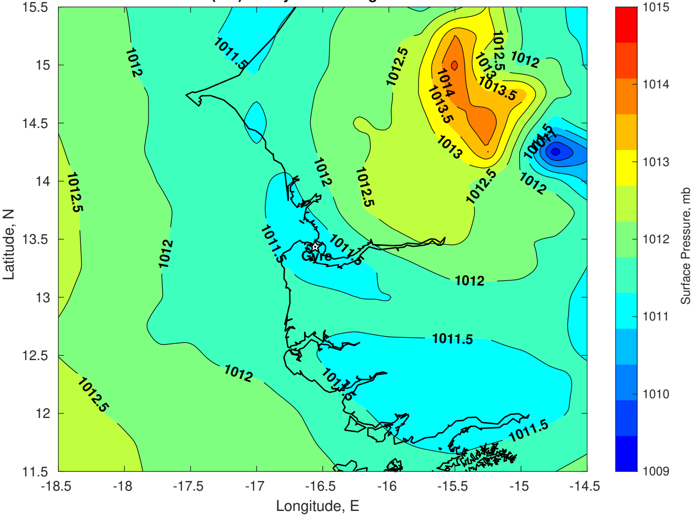
Surface Pressure (mb) for Gyre at 08-Aug-2025 00:00:00
