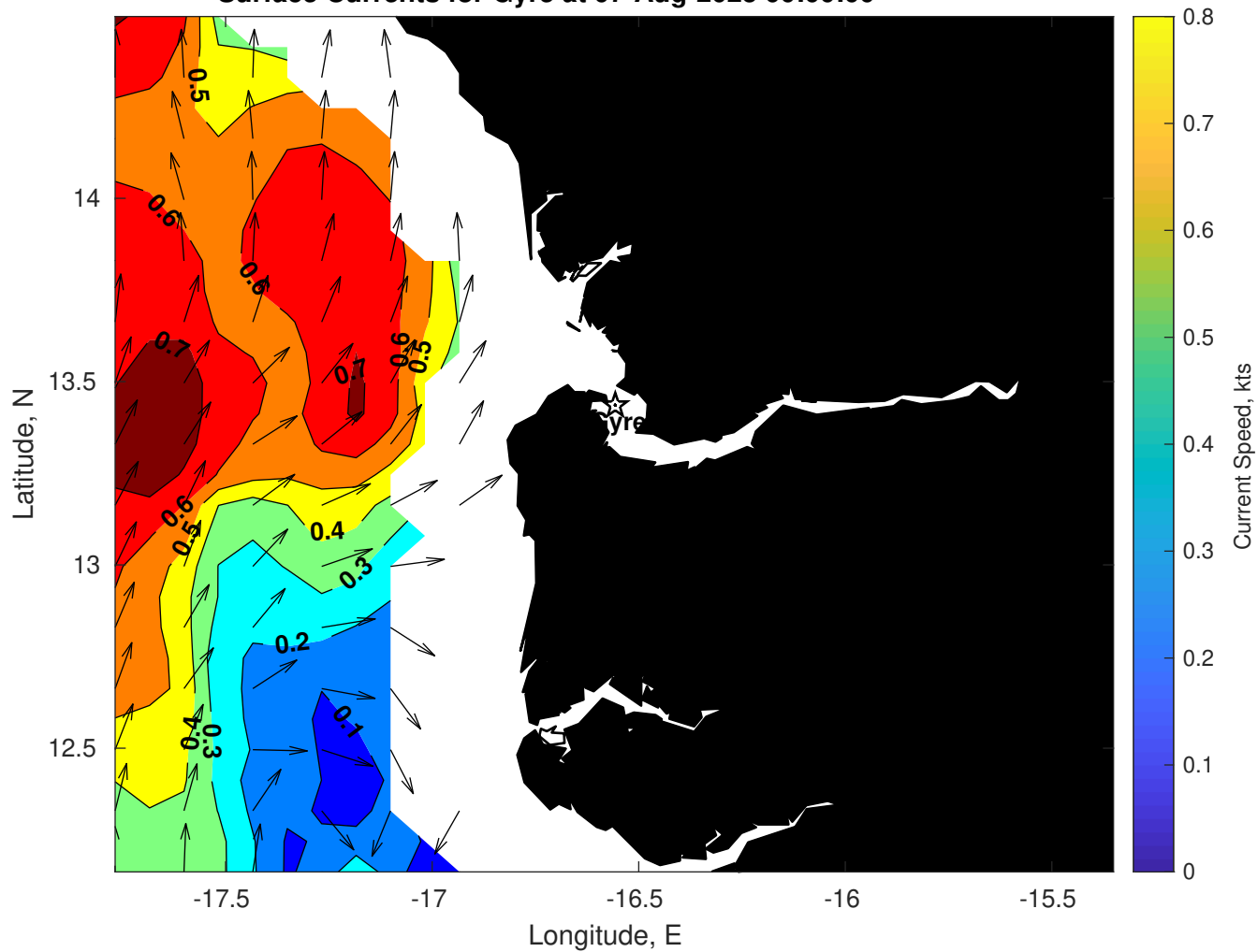
Surface Currents for Gyre at 07-Aug-2025 00:00:00
