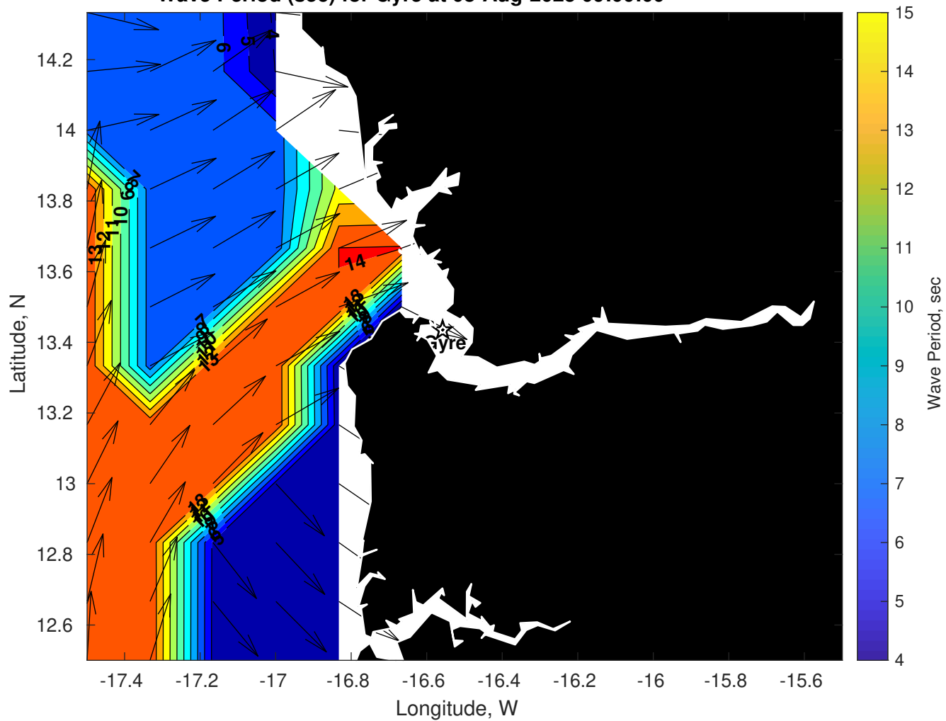
Wave Period (sec) for Gyre at 08-Aug-2025 09:00:00
