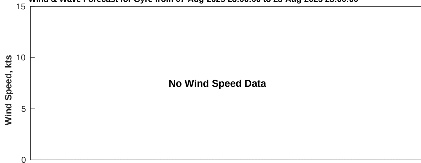
Wind & Wave Forecast for Gyre from 07-Aug-2025 23:00:00 to 23-Aug-2025 23:00:00
