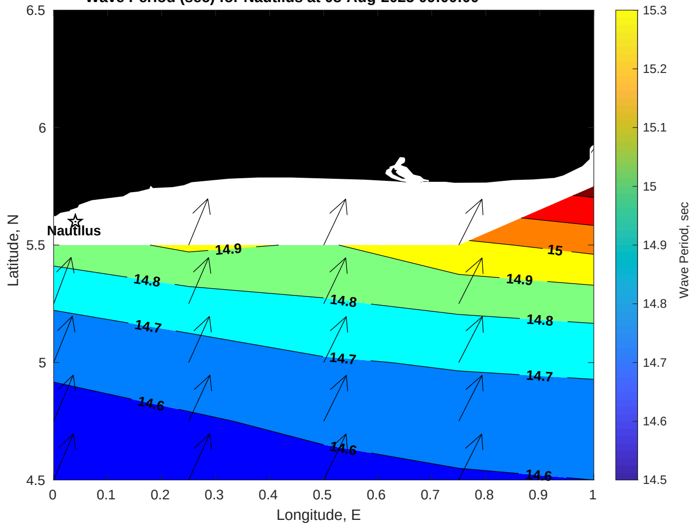
Wave Period (sec) for Nautilus at 08-Aug-2025 09:00:00
