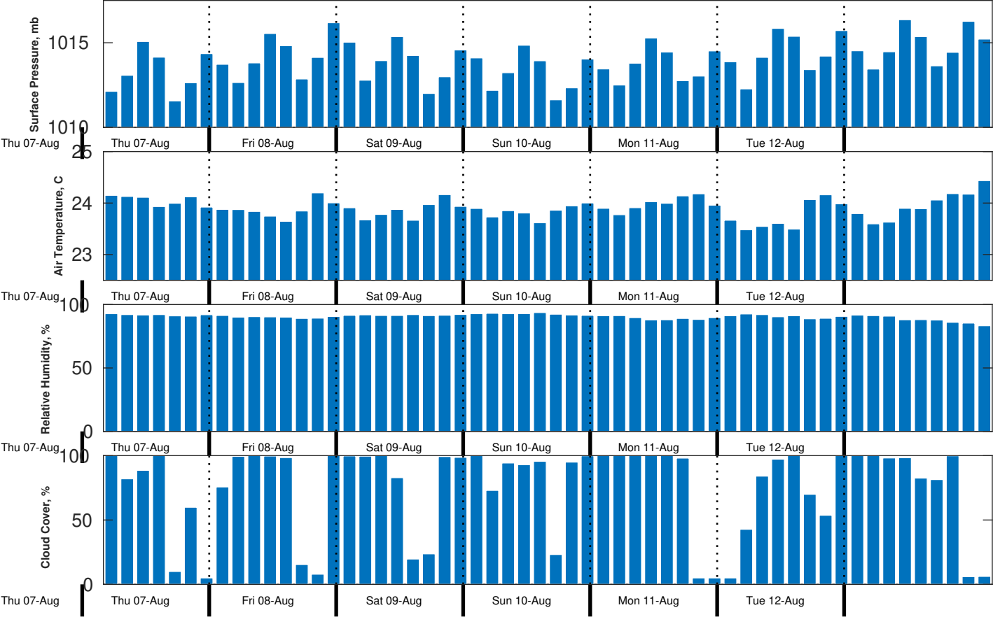
Met Forecast for Nautilus from 08-Aug-2025 00:00:00 to 15-Aug-2025 00:00:00
