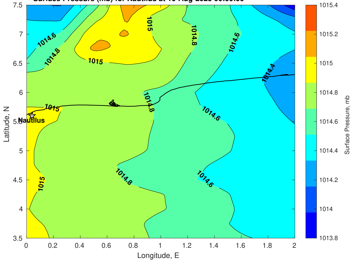
Surface Pressure (mb) for Nautilus at 10-Aug-2025 00:00:00
