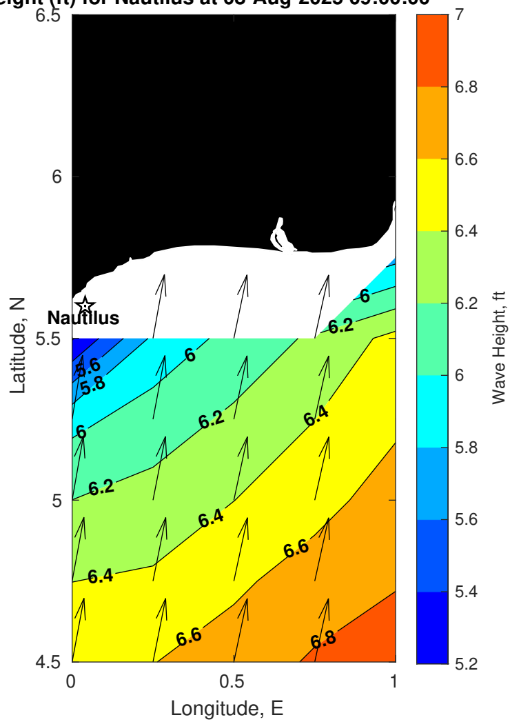
Wave Height (ft) for Nautilus at 08-Aug-2025 09:00:00
