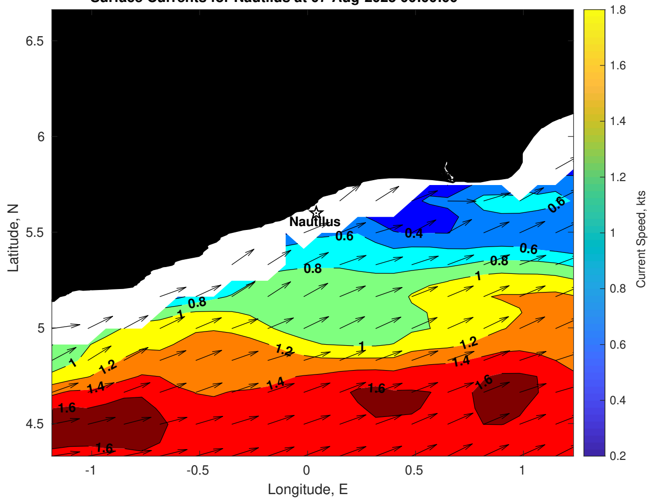
Surface Currents for Nautilus at 07-Aug-2025 00:00:00
