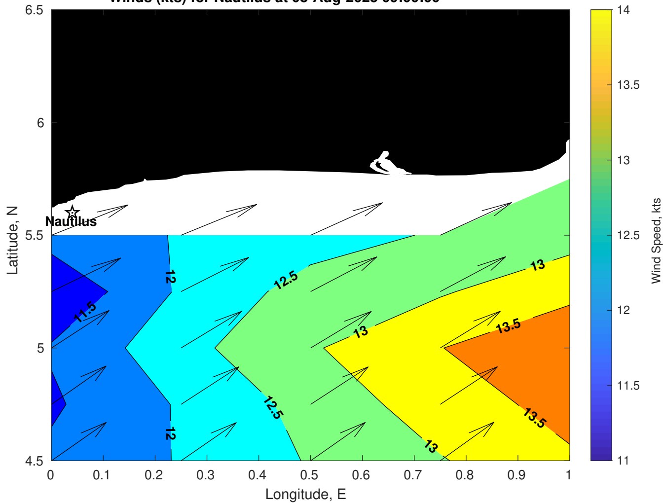
Winds (kts) for Nautilus at 08-Aug-2025 09:00:00
