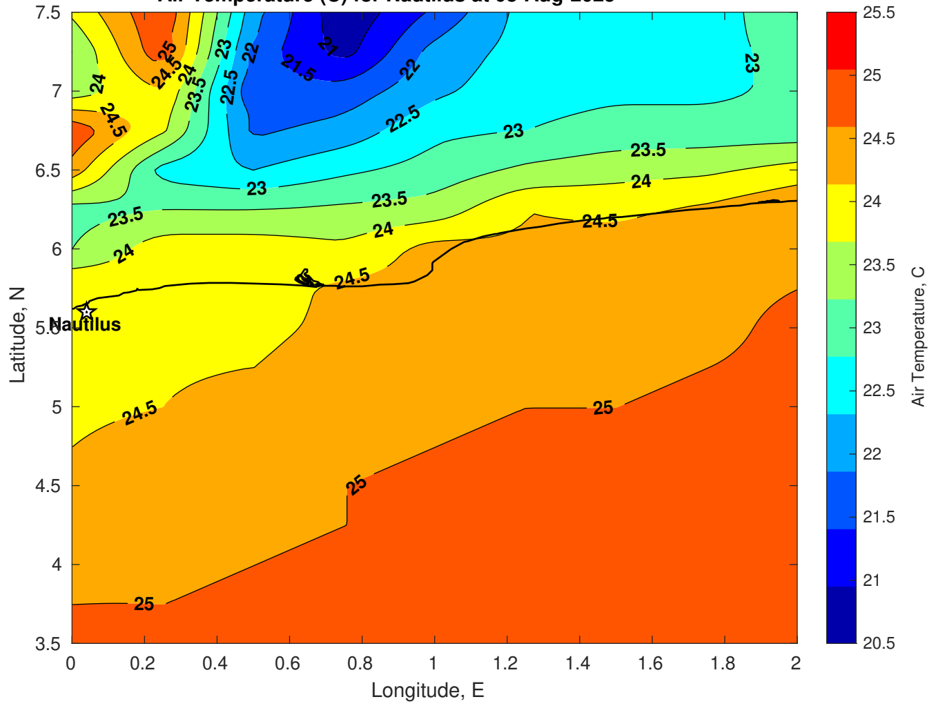
Air Temperature (C) for Nautilus at 08-Aug-2025
