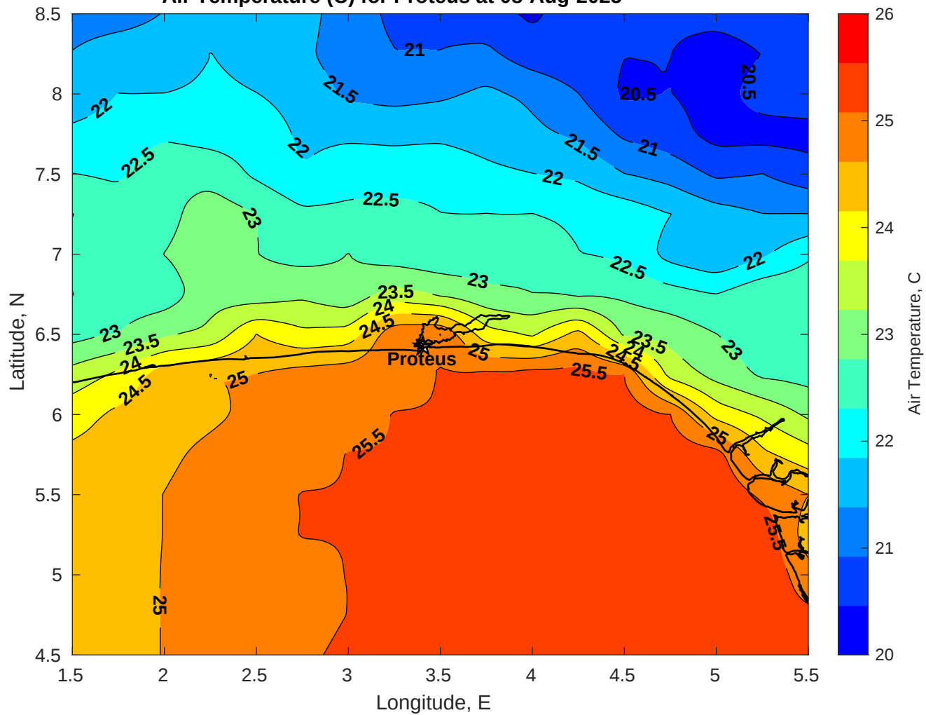
Air Temperature (C) for Proteus at 08-Aug-2025
