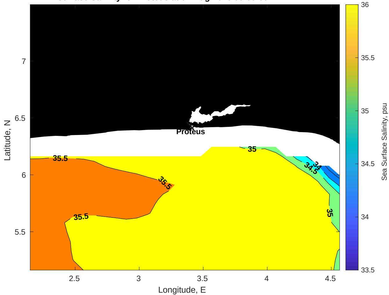
Surface Salinity for Proteus at 07-Aug-2025 00:00:00
