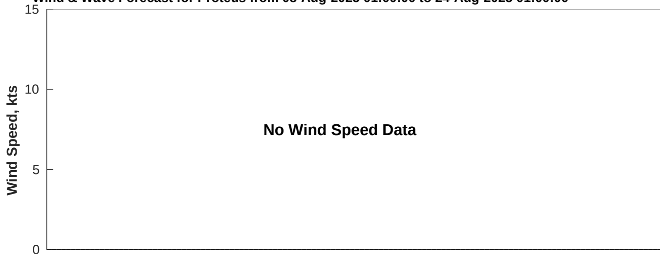
Wind & Wave Forecast for Proteus from 08-Aug-2025 01:00:00 to 24-Aug-2025 01:00:00
