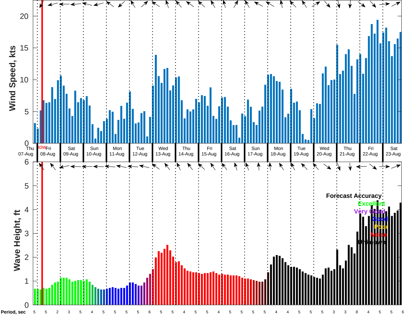
Wind & Wave Forecast for Shell Noches GC19 PPL Geotechnical from 07-Aug-2025 20:00:00 to 23-Aug-2025 20:00:00
