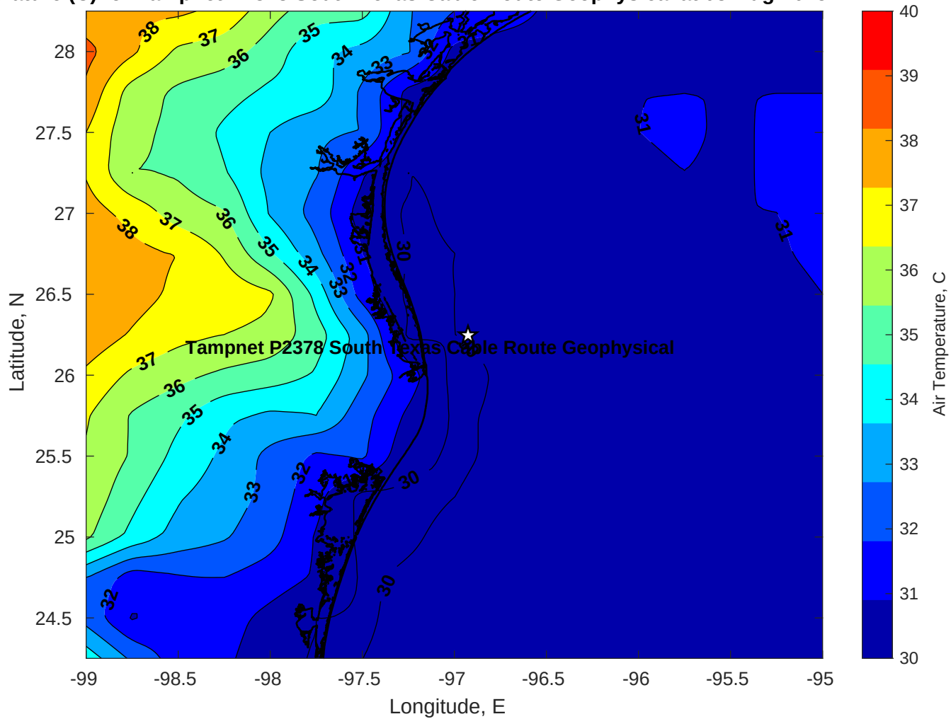
Air Temperature (C) for Tampnet P2378 South Texas Cable Route Geophysical at 08-Aug-2025
