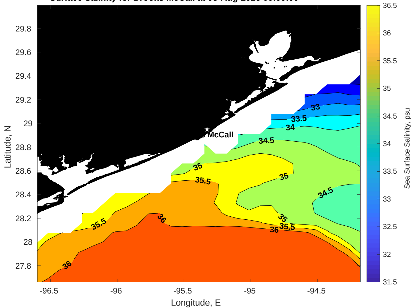
Surface Salinity for Brooks McCall at 08-Aug-2025 00:00:00
