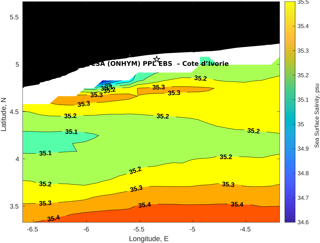
Surface Salinity for CSA (ONHYM) PPL EBS - Cote d'Ivoire at 08-Aug-2025 00:00:00
