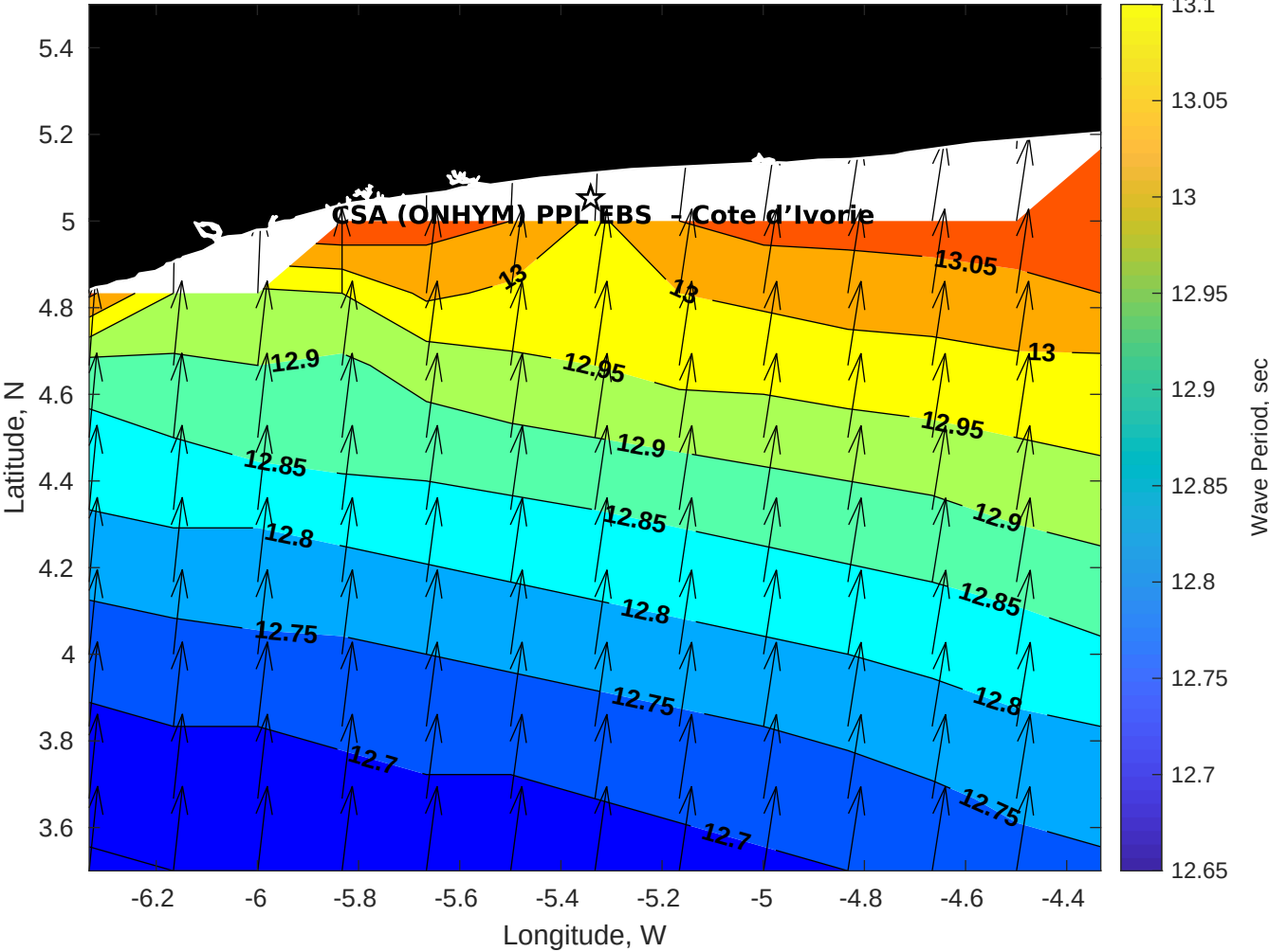
Wave Period (sec) for CSA (ONHYM) PPL EBS - Cote d'Ivoire at 09-Aug-2025 09:00:00
