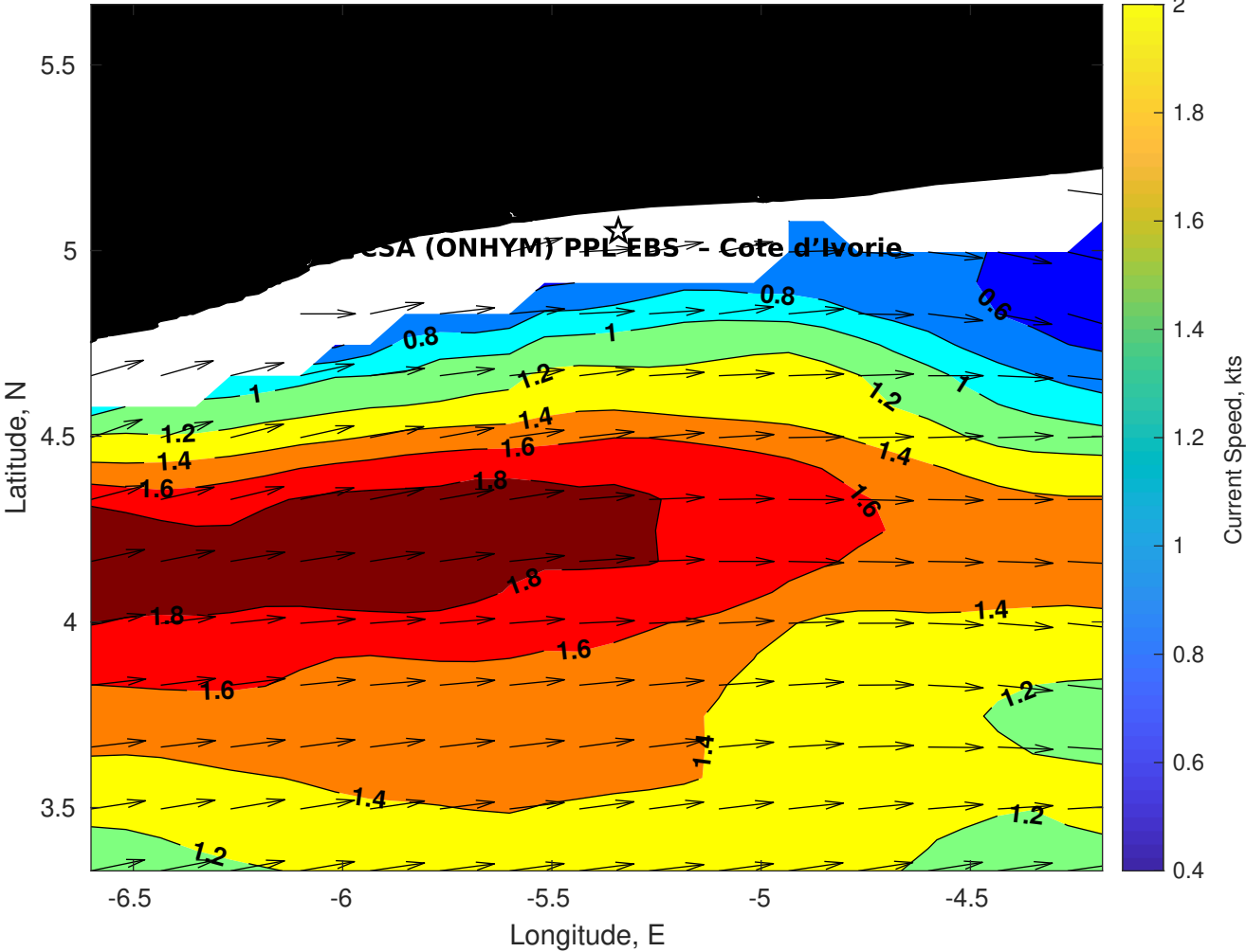
Surface Currents for CSA (ONHYM) PPL EBS - Cote d'Ivoire at 08-Aug-2025 00:00:00
