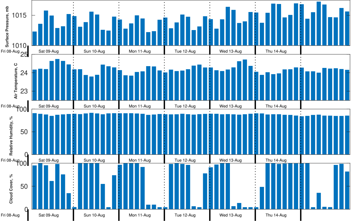
Met Forecast for CSA (ONHYM) PPL EBS - Cote d'Ivoire from 09-Aug-2025 00:00:00 to 16-Aug-2025 00:00:00
