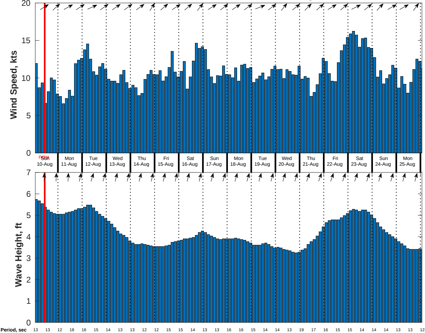
Wind & Wave Forecast for CSA (ONHYM) PPL EBS - Cote d'Ivoire from 09-Aug-2025 01:00:00 to 25-Aug-2025 01:00:00
