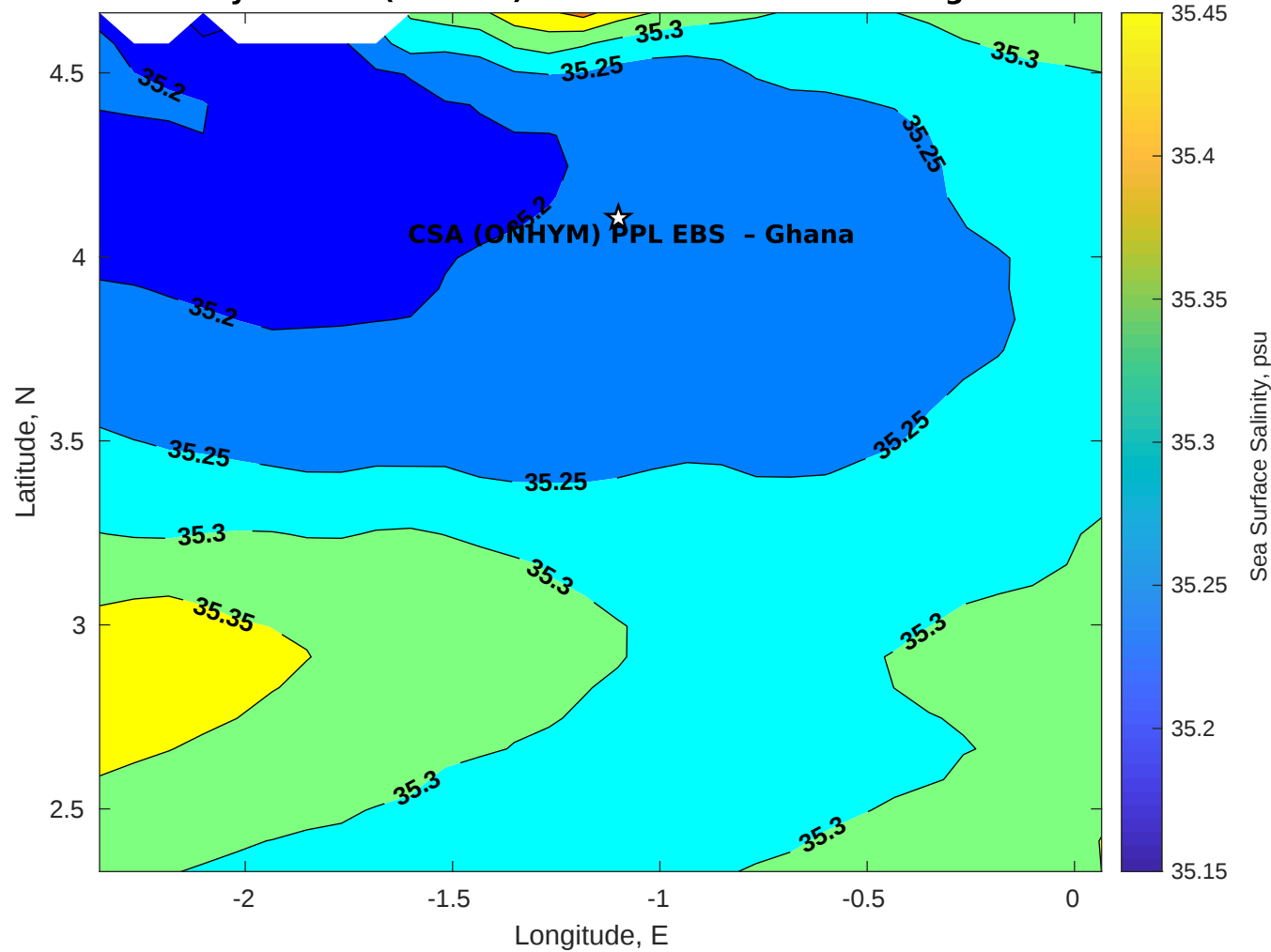
Surface Salinity for CSA (ONHYM) PPL EBS - Ghana at 08-Aug-2025 00:00:00
