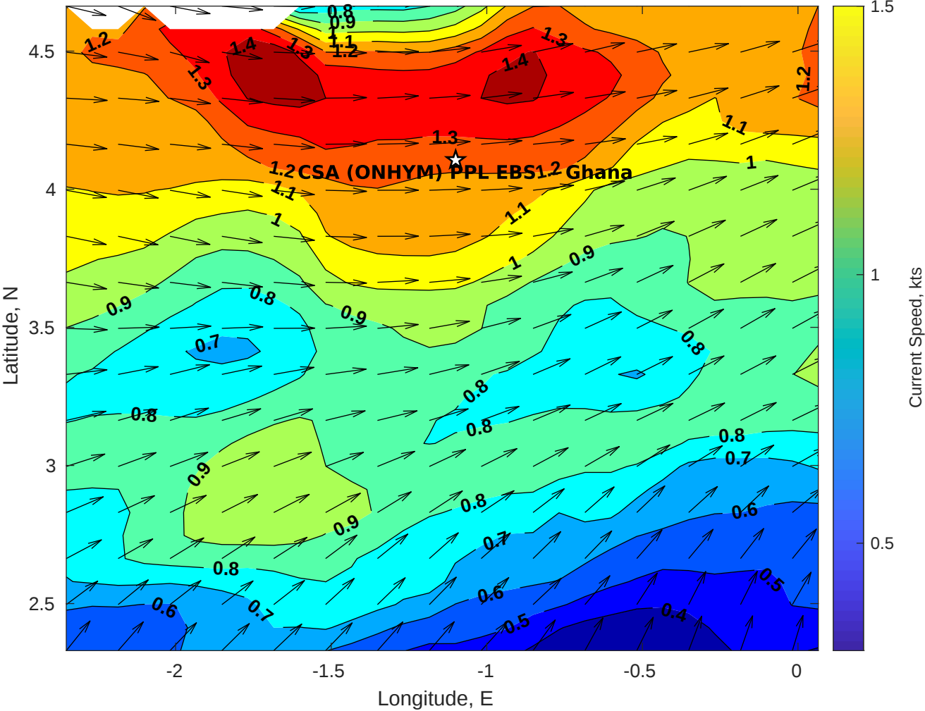
Surface Currents for CSA (ONHYM) PPL EBS - Ghana at 08-Aug-2025 00:00:00
