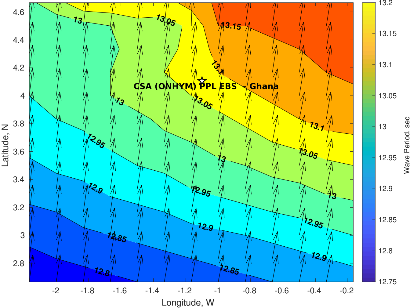
Wave Period (sec) for CSA (ONHYM) PPL EBS - Ghana at 09-Aug-2025 09:00:00
