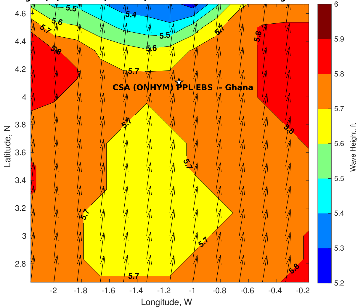
Wave Height (ft) for CSA (ONHYM) PPL EBS - Ghana at 09-Aug-2025 09:00:00
