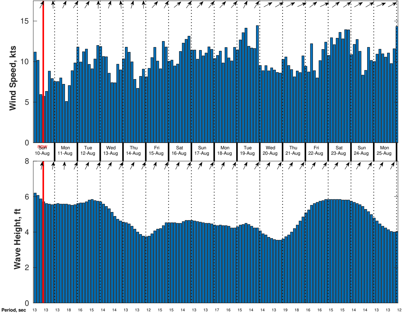
Wind & Wave Forecast for CSA (ONHYM) PPL EBS - Ghana from 09-Aug-2025 02:00:00 to 25-Aug-2025 02:00:00
