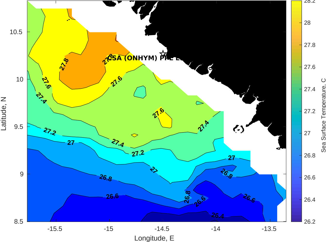
SST for CSA (ONHYM) PPL EBS - Guinea at 08-Aug-2025 00:00:00
