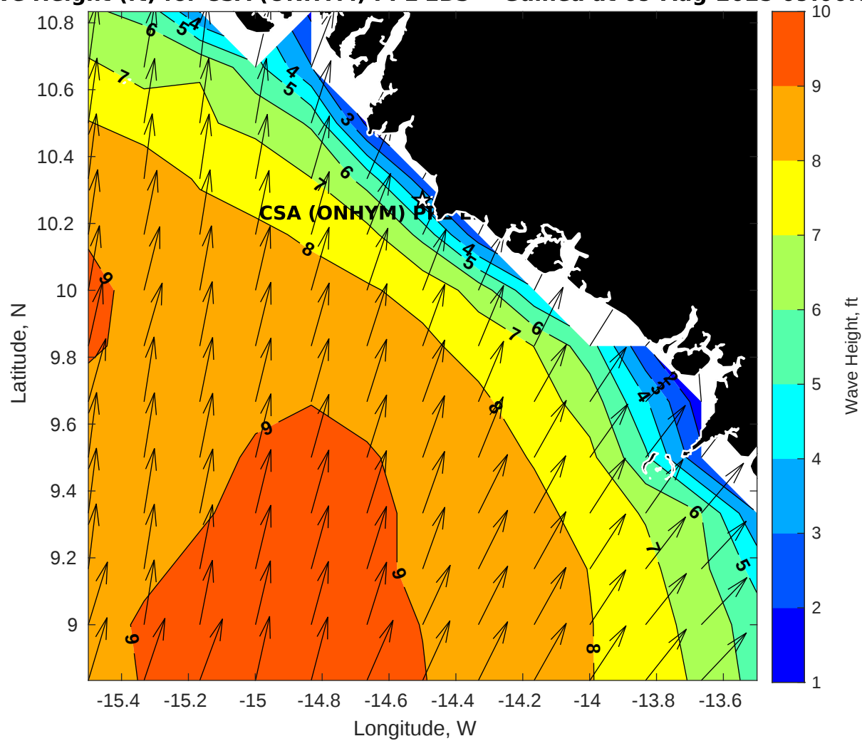
Wave Height (ft) for CSA (ONHYM) PPL EBS - Guinea at 09-Aug-2025 09:00:00
