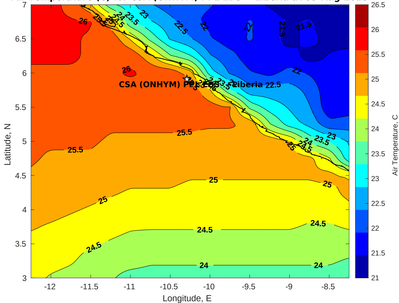
Air Temperature (C) for CSA (ONHYM) PPL EBS - Liberia at 09-Aug-2025
