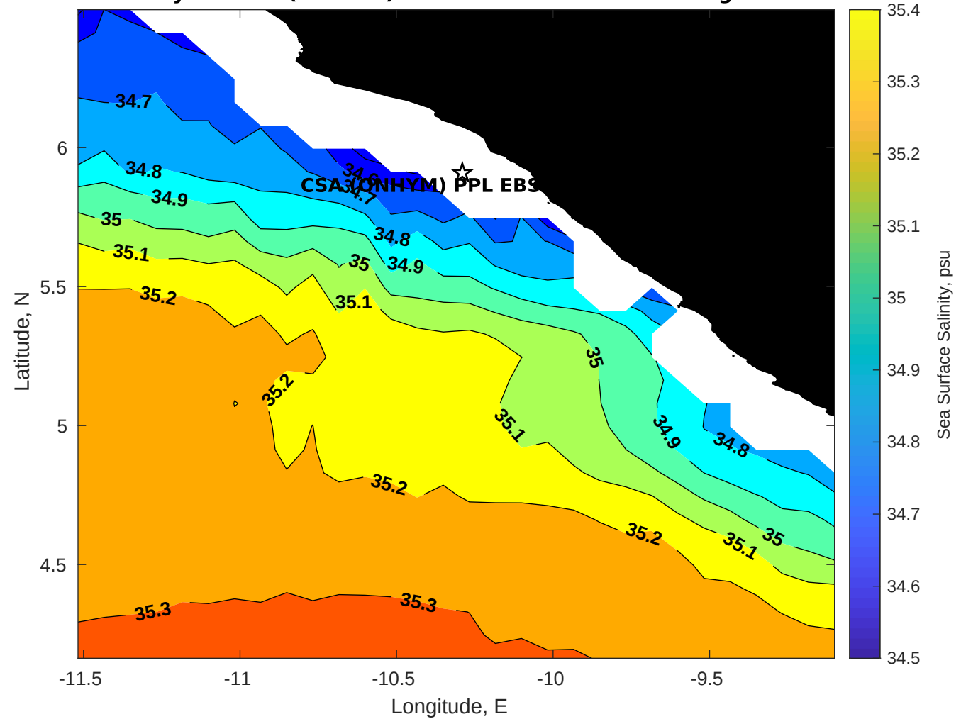
Surface Salinity for CSA (ONHYM) PPL EBS - Liberia at 08-Aug-2025 00:00:00
