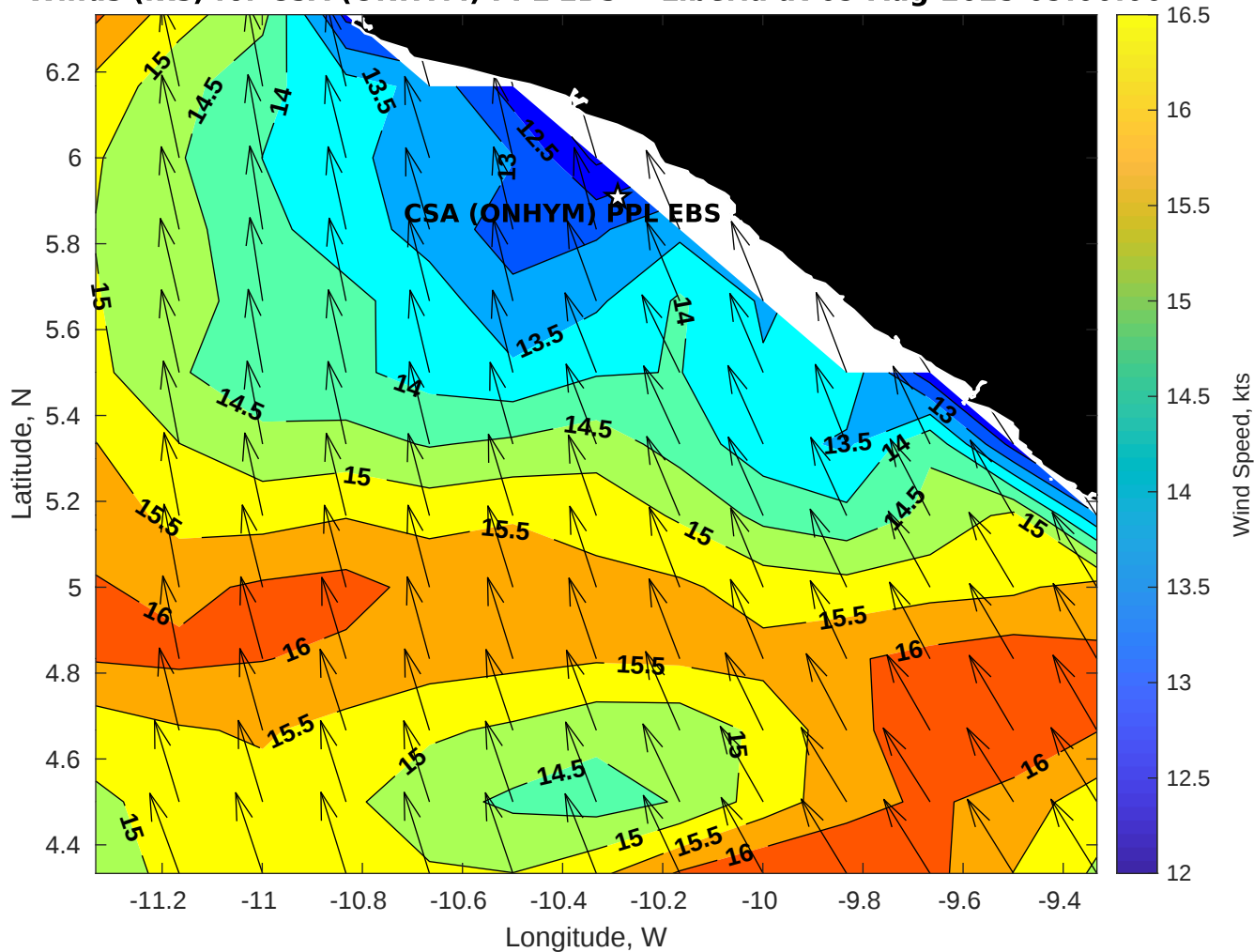
Winds (kts) for CSA (ONHYM) PPL EBS - Liberia at 09-Aug-2025 09:00:00
