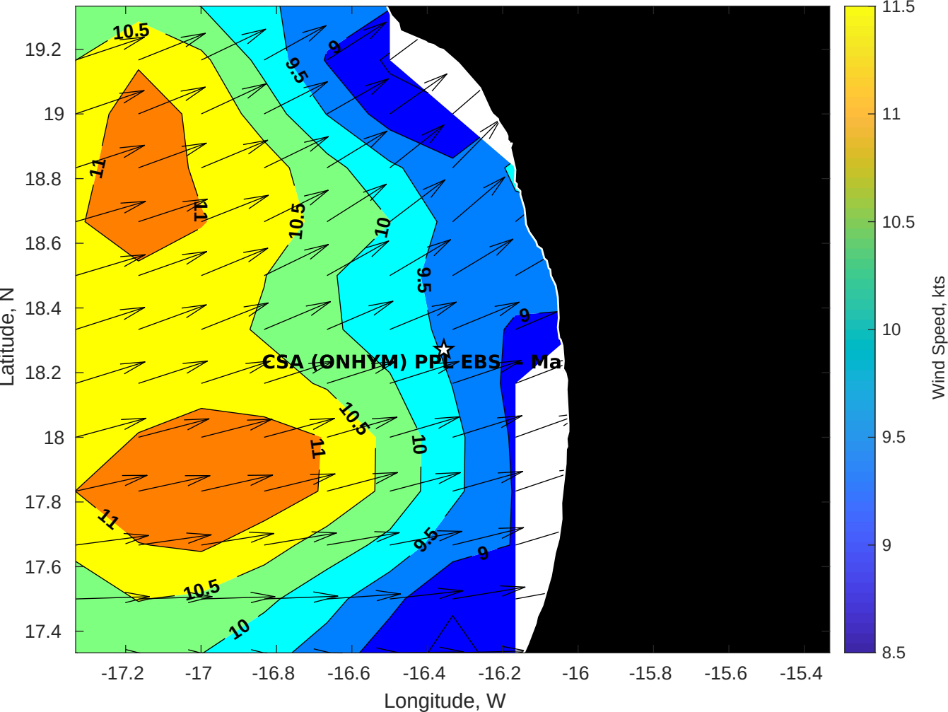
Winds (kts) for CSA (ONHYM) PPL EBS - Mauritania at 09-Aug-2025 09:00:00
