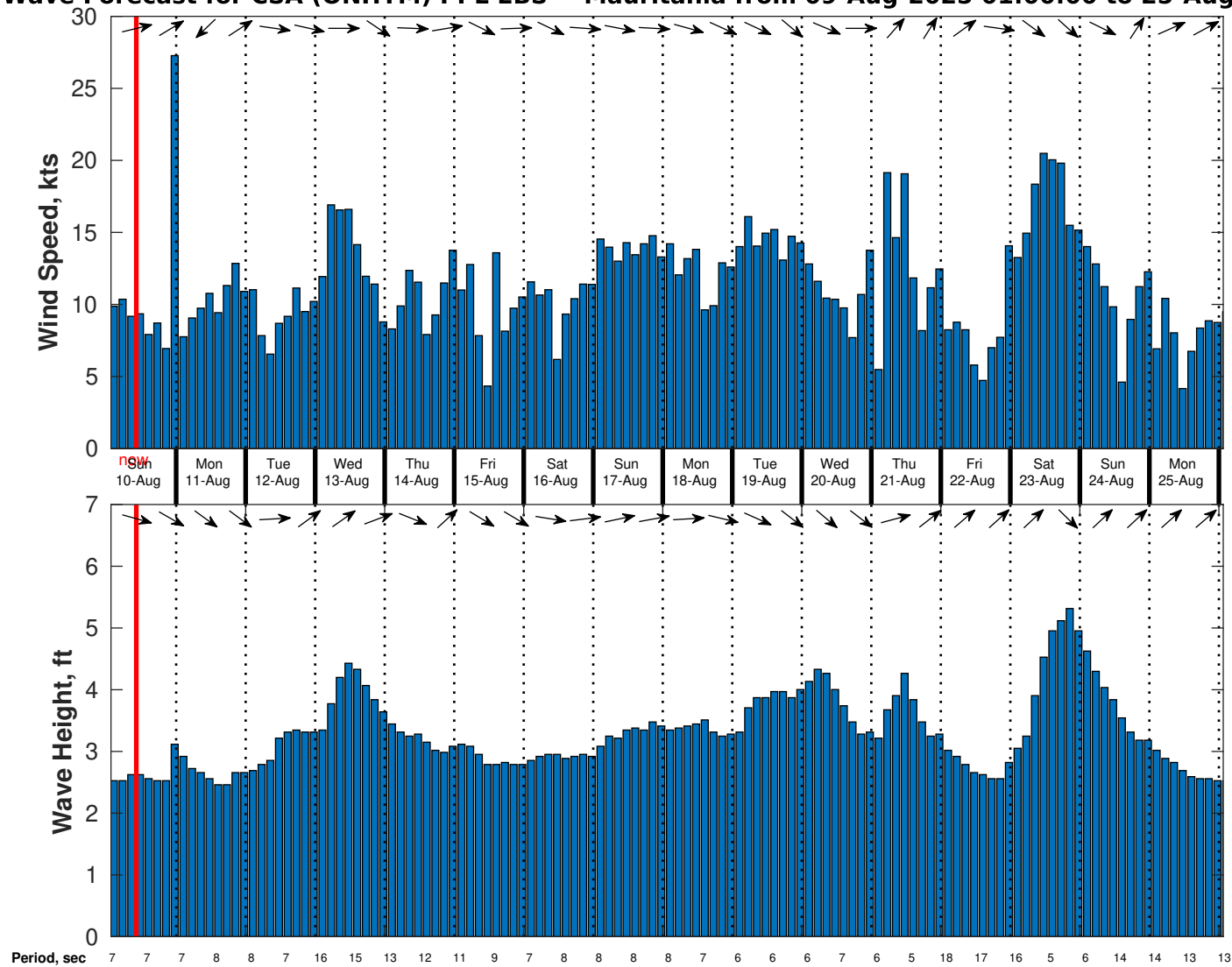
Wind & Wave Forecast for CSA (ONHYM) PPL EBS - Mauritania from 09-Aug-2025 01:00:00 to 25-Aug-2025 01:00:00
