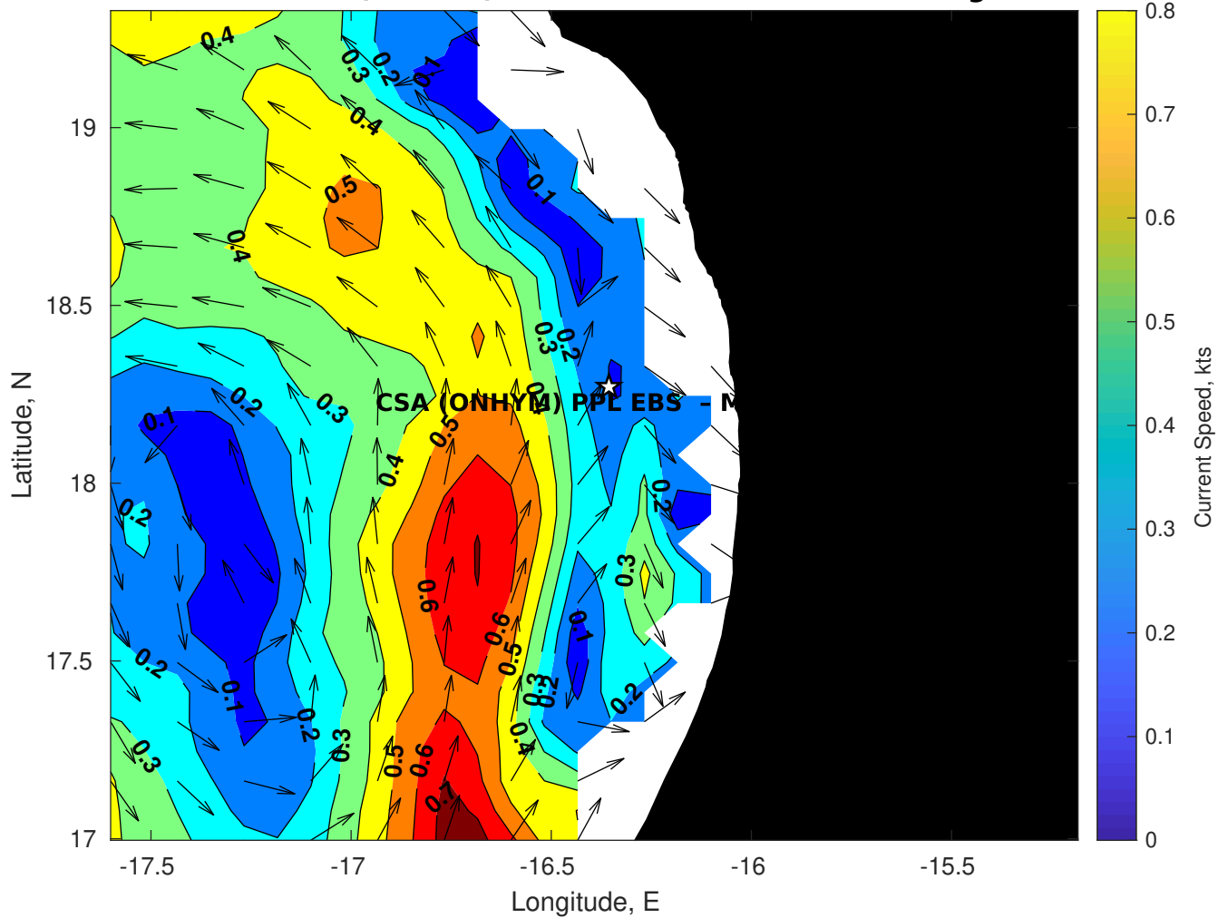
Surface Currents for CSA (ONHYM) PPL EBS - Mauritania at 08-Aug-2025 00:00:00
