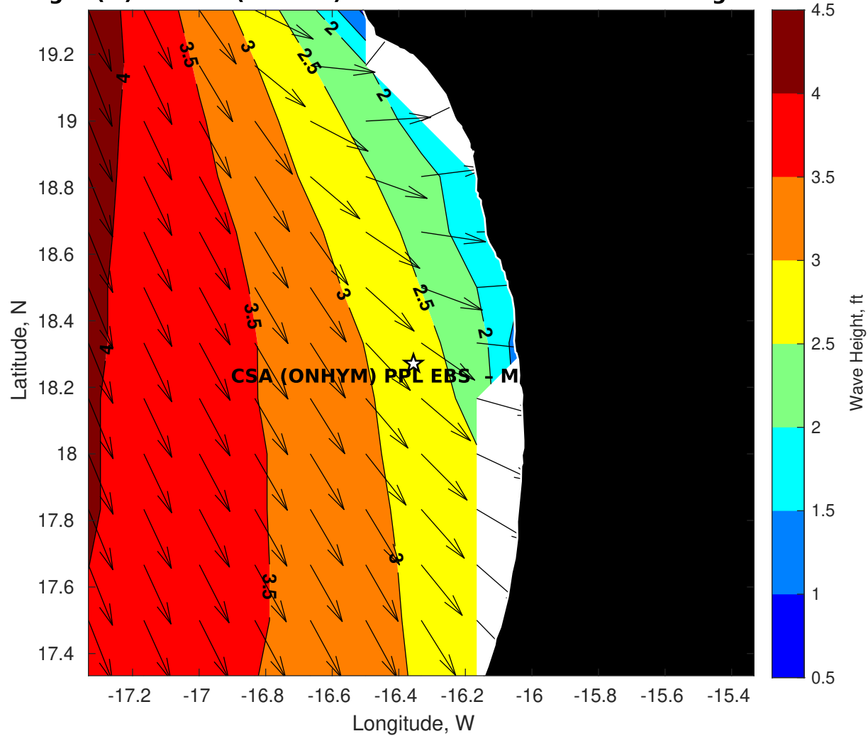
Wave Height (ft) for CSA (ONHYM) PPL EBS - Mauritania at 09-Aug-2025 09:00:00
