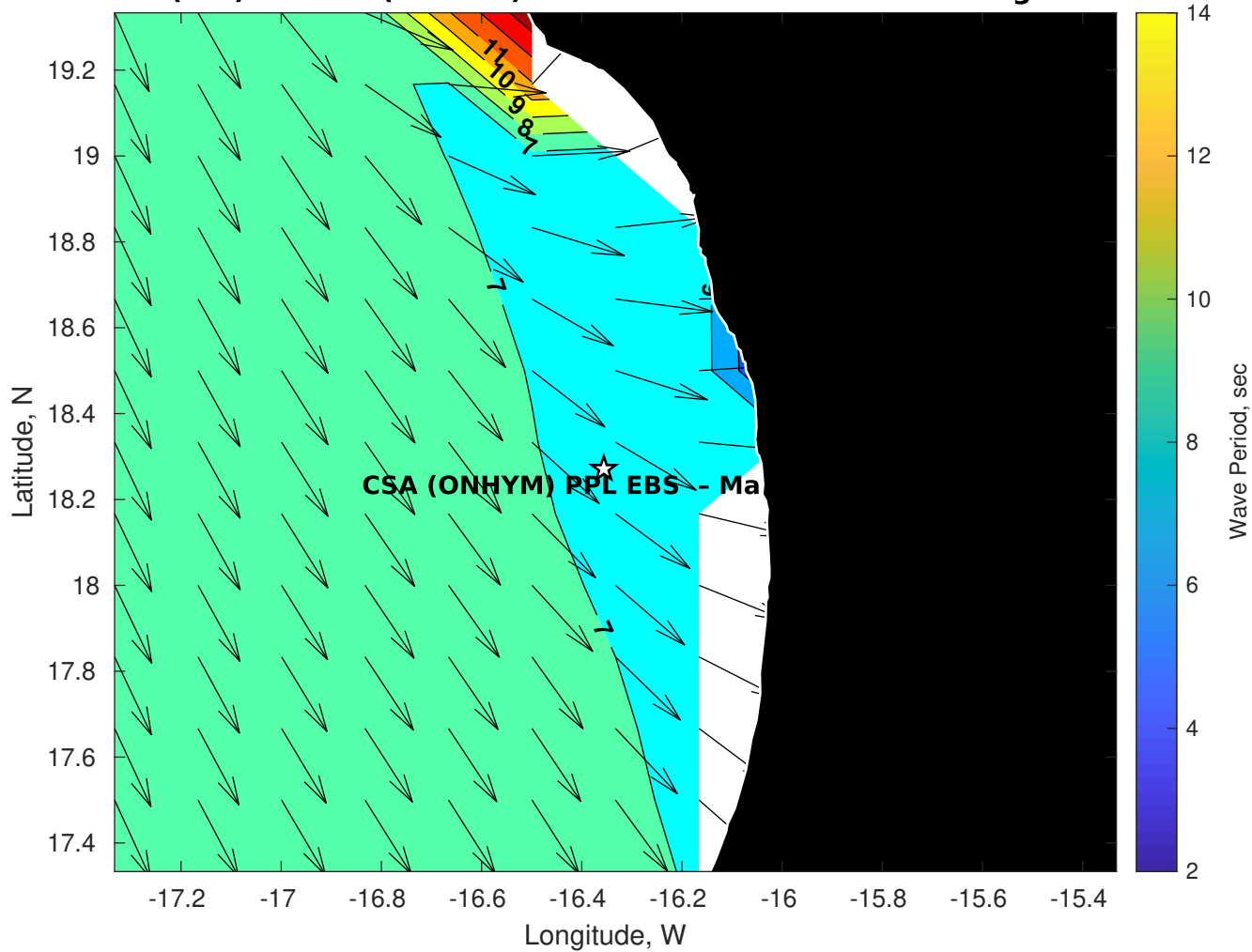
Wave Period (sec) for CSA (ONHYM) PPL EBS - Mauritania at 09-Aug-2025 09:00:00
