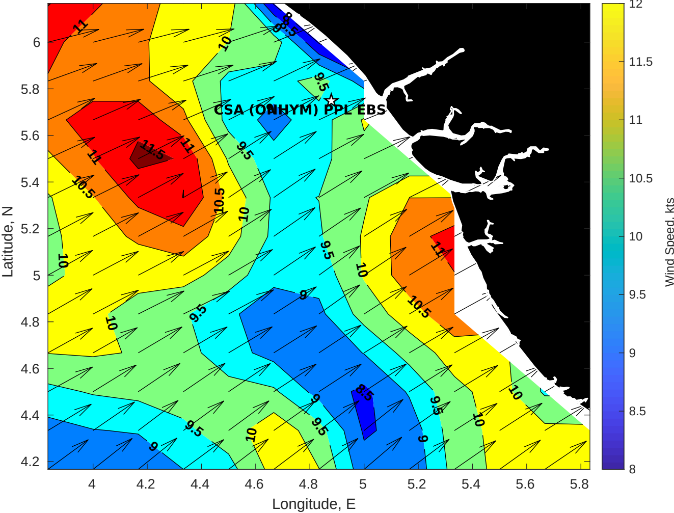
Winds (kts) for CSA (ONHYM) PPL EBS - Nigeria at 09-Aug-2025 09:00:00
