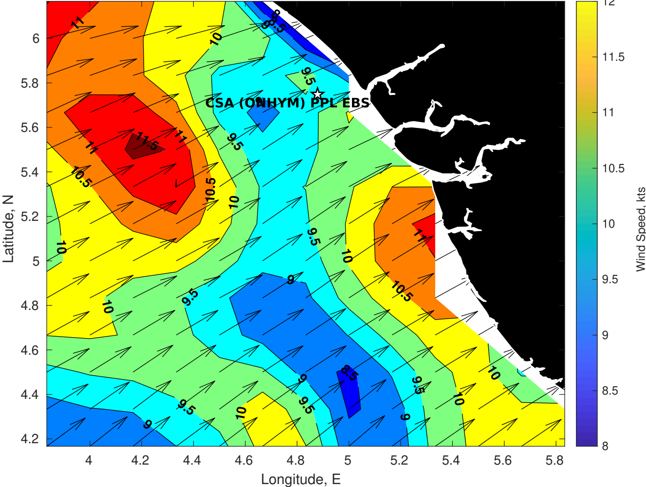
Winds (kts) for CSA (ONHYM) PPL EBS - Nigeria at 09-Aug-2025 09:00:00
