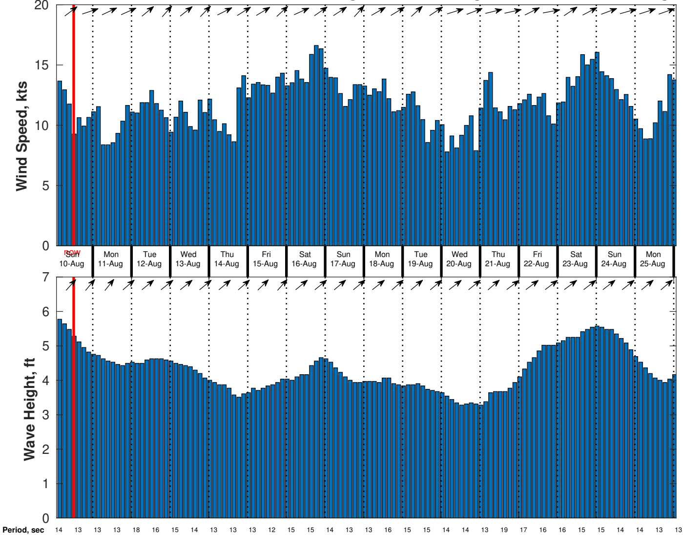
Wind & Wave Forecast for CSA (ONHYM) PPL EBS - Nigeria from 09-Aug-2025 02:00:00 to 25-Aug-2025 02:00:00
