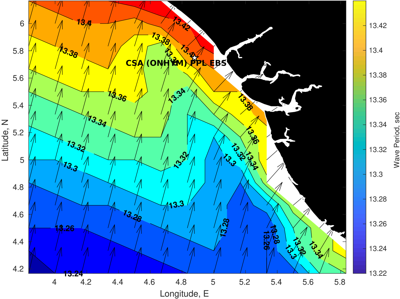
Wave Period (sec) for CSA (ONHYM) PPL EBS - Nigeria at 09-Aug-2025 09:00:00
