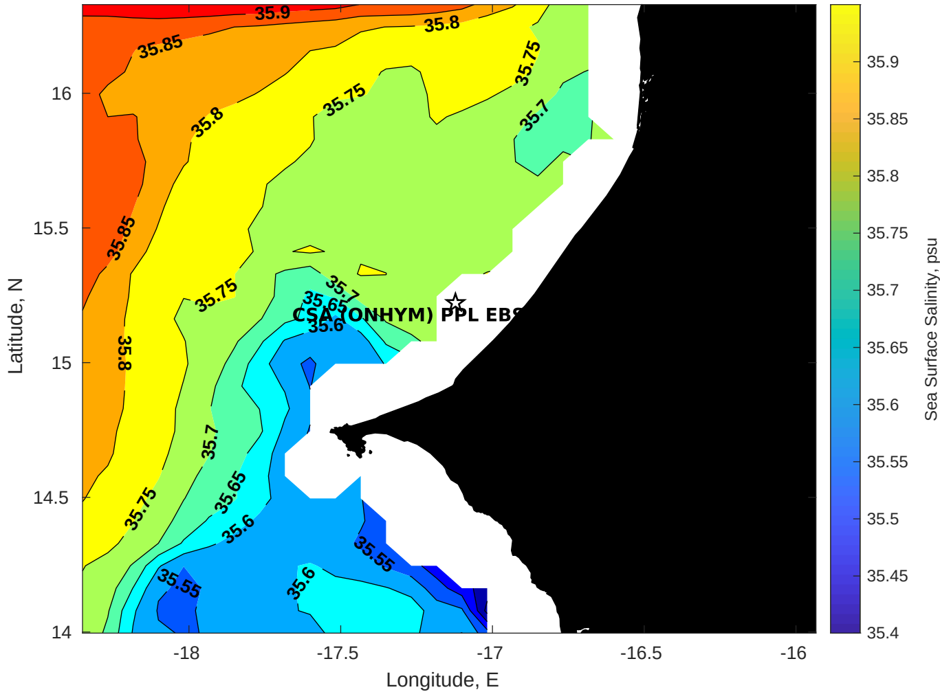
Surface Salinity for CSA (ONHYM) PPL EBS - Senegal at 08-Aug-2025 00:00:00
