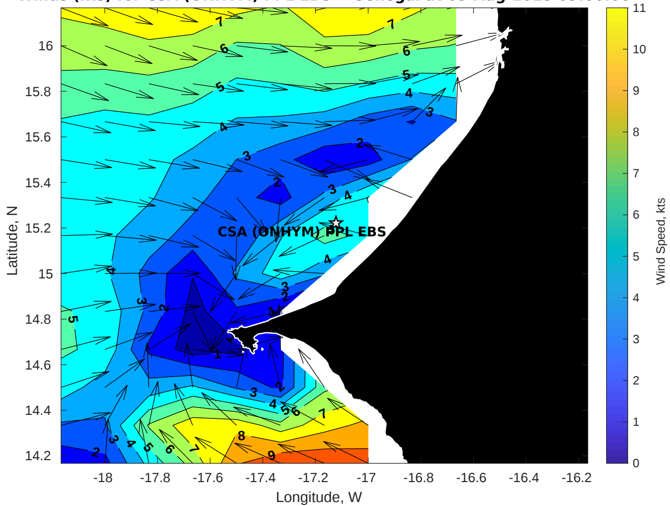
Winds (kts) for CSA (ONHYM) PPL EBS - Senegal at 09-Aug-2025 09:00:00
