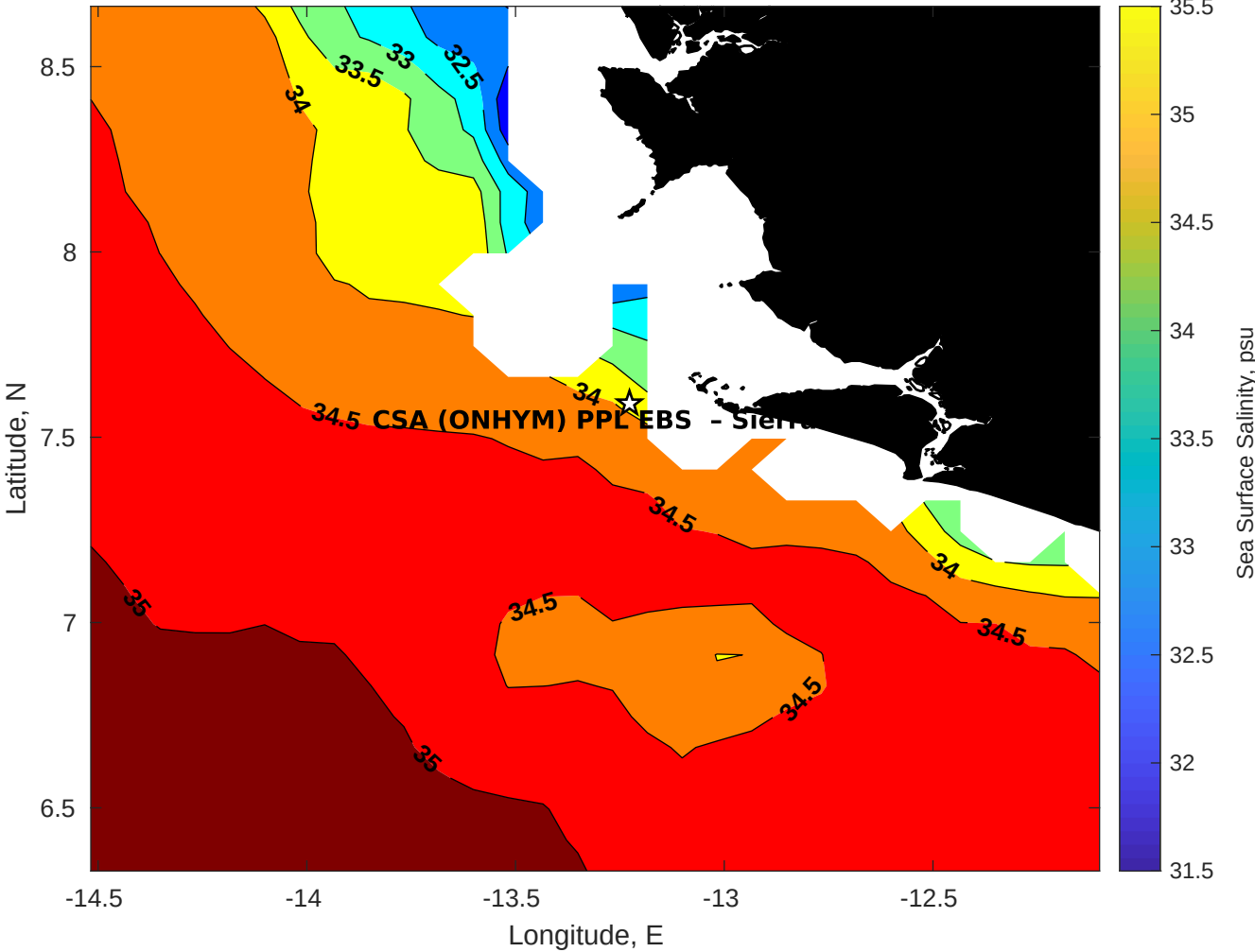
Surface Salinity for CSA (ONHYM) PPL EBS - Sierra Leone at 08-Aug-2025 00:00:00
