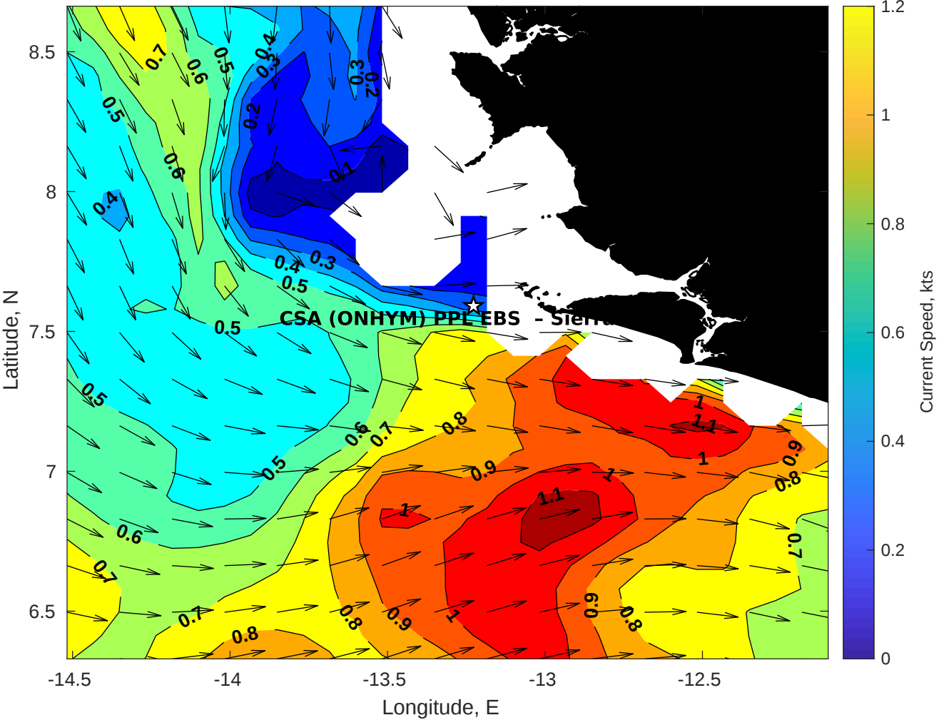
Surface Currents for CSA (ONHYM) PPL EBS - Sierra Leone at 08-Aug-2025 00:00:00
