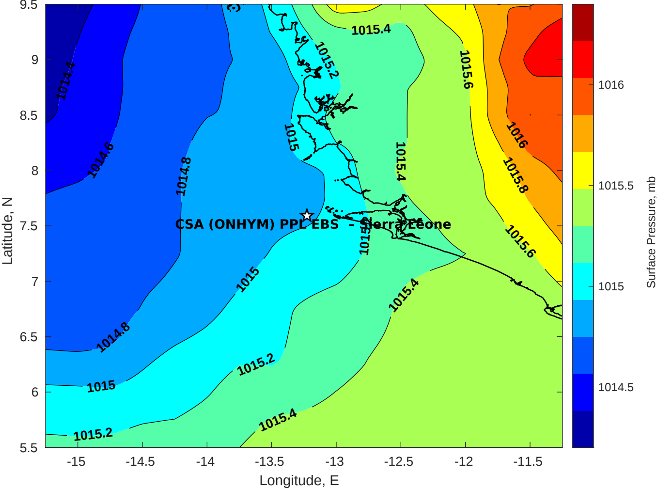
Surface Pressure (mb) for CSA (ONHYM) PPL EBS - Sierra Leone at 10-Aug-2025 00:00:00
