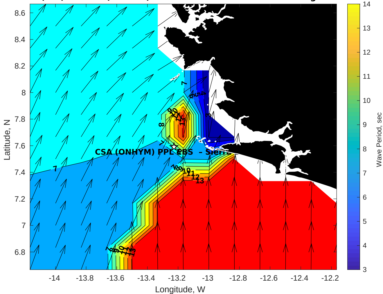
Wave Period (sec) for CSA (ONHYM) PPL EBS - Sierra Leone at 09-Aug-2025 09:00:00
