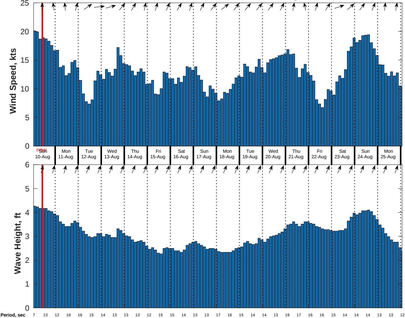
Wind & Wave Forecast for CSA (ONHYM) PPL EBS - Sierra Leone from 09-Aug-2025 01:00:00 to 25-Aug-2025 01:00:00
