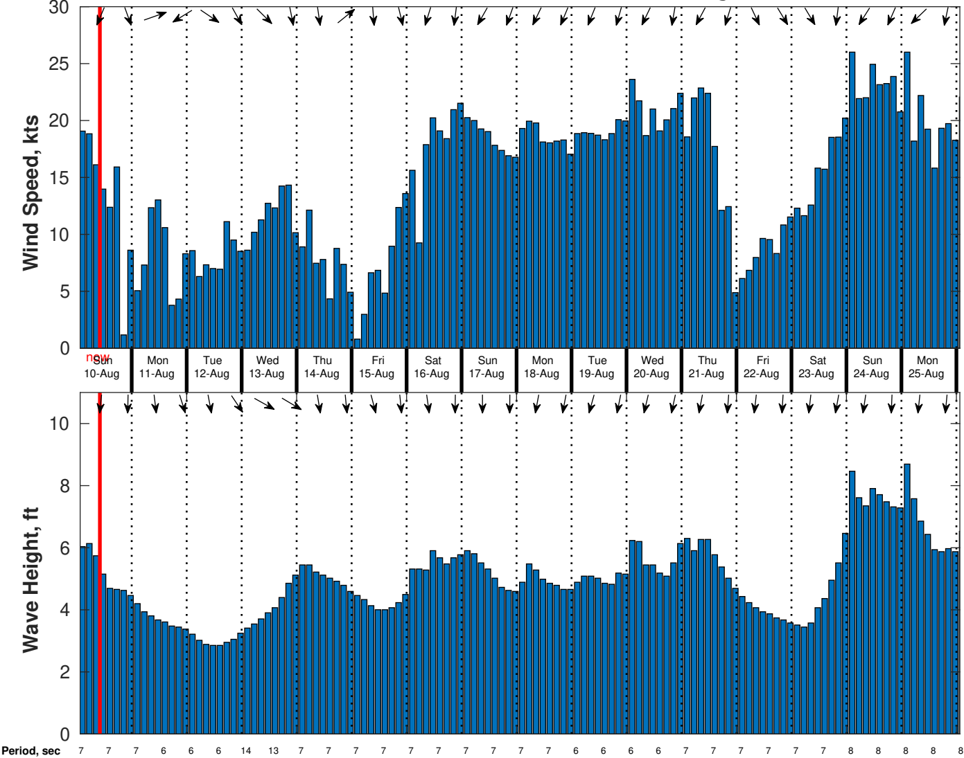
Wind & Wave Forecast for CSA (ONHYM) PPL EBS - Western Sahara from 09-Aug-2025 01:00:00 to 25-Aug-2025 01:00:00
