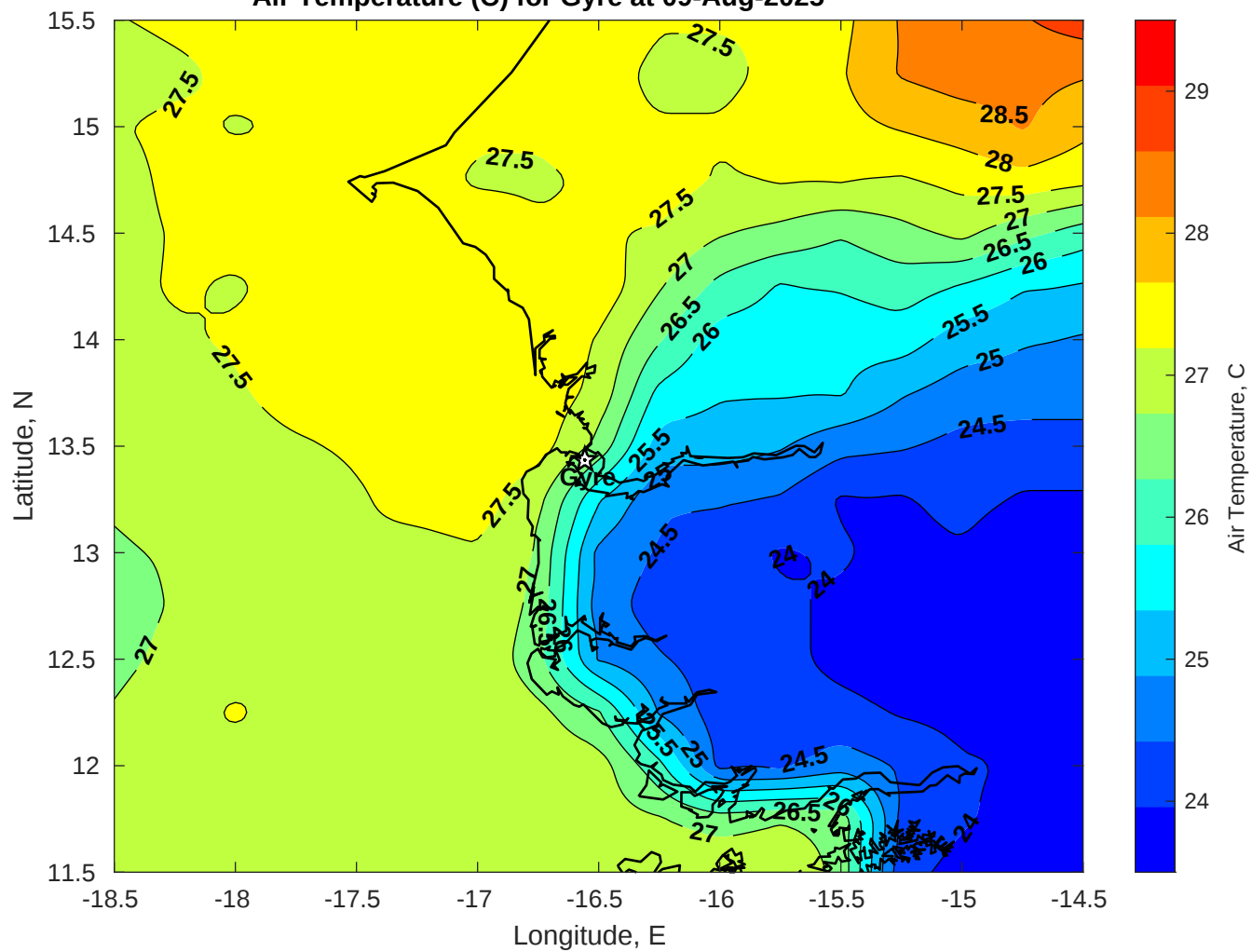
Air Temperature (C) for Gyre at 09-Aug-2025
