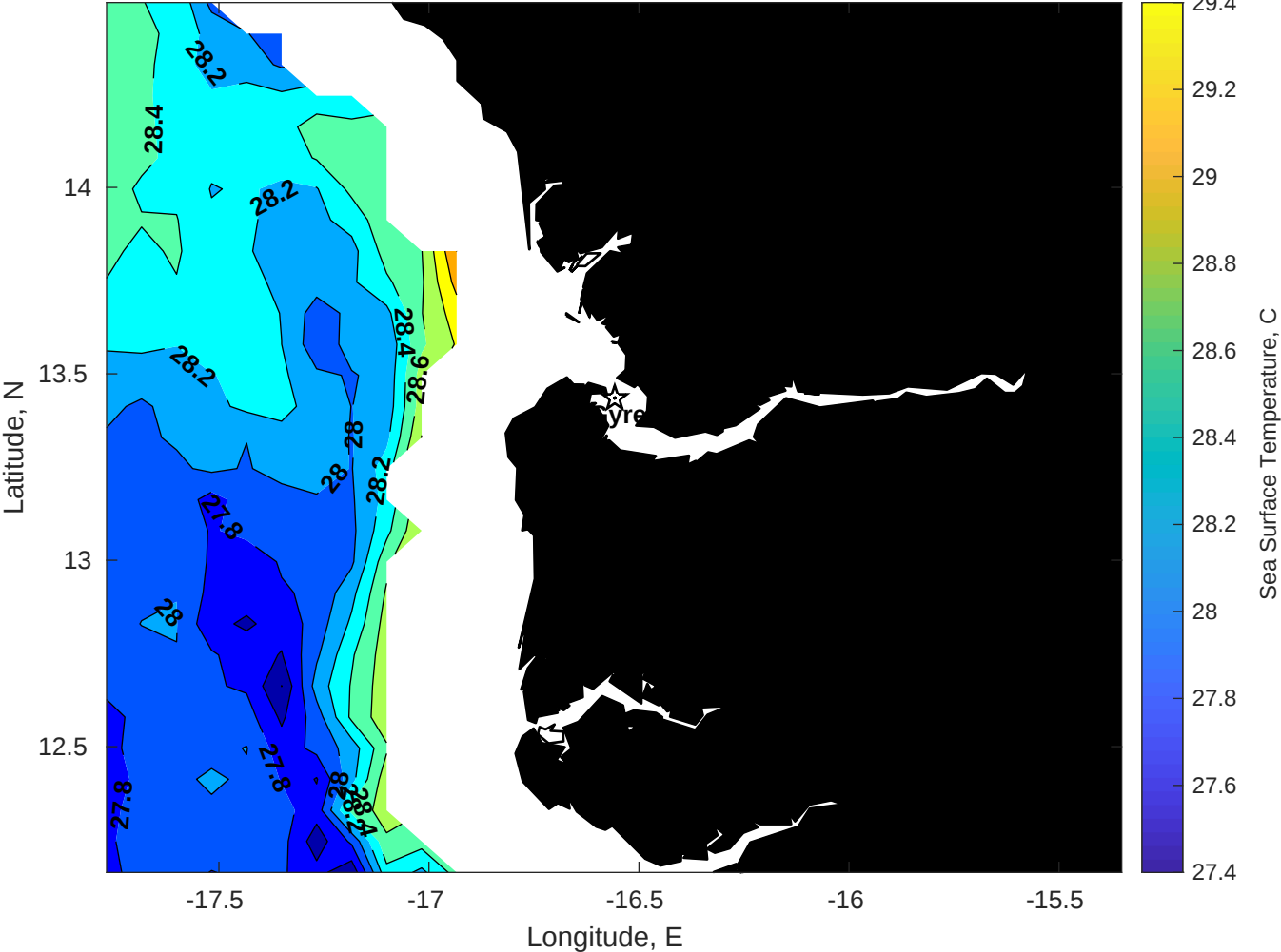
SST for Gyre at 08-Aug-2025 00:00:00
