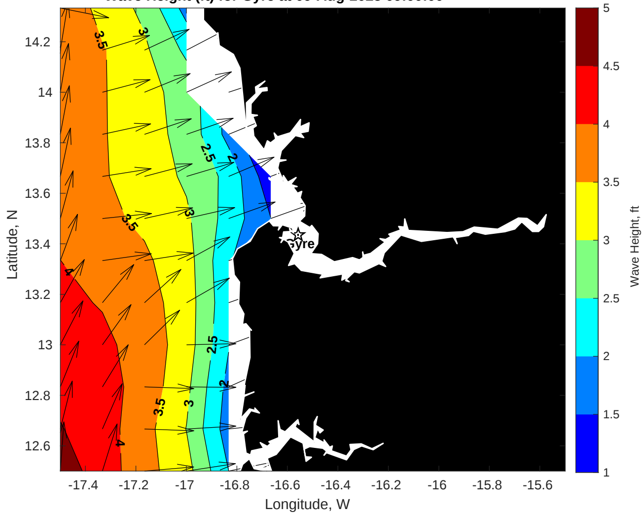
Wave Height (ft) for Gyre at 09-Aug-2025 09:00:00
