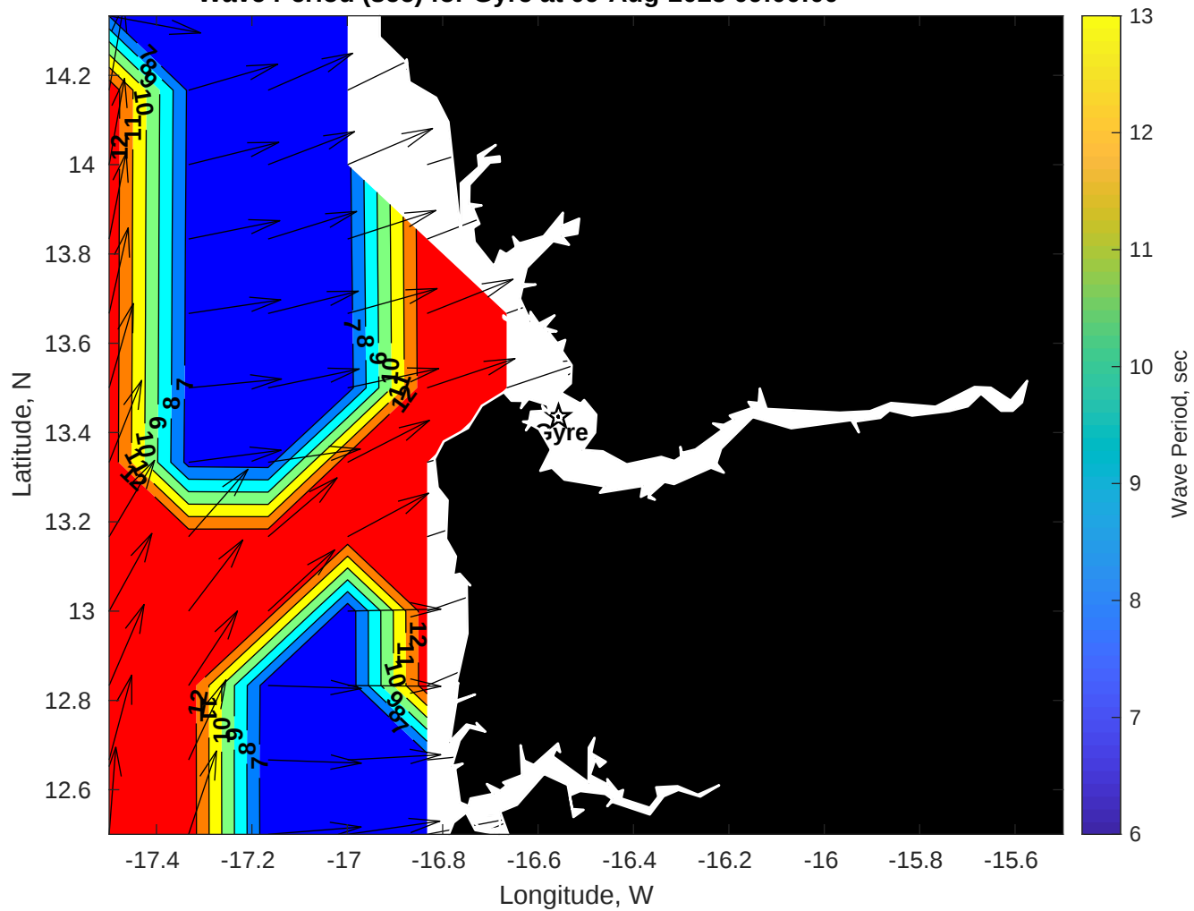
Wave Period (sec) for Gyre at 09-Aug-2025 09:00:00
