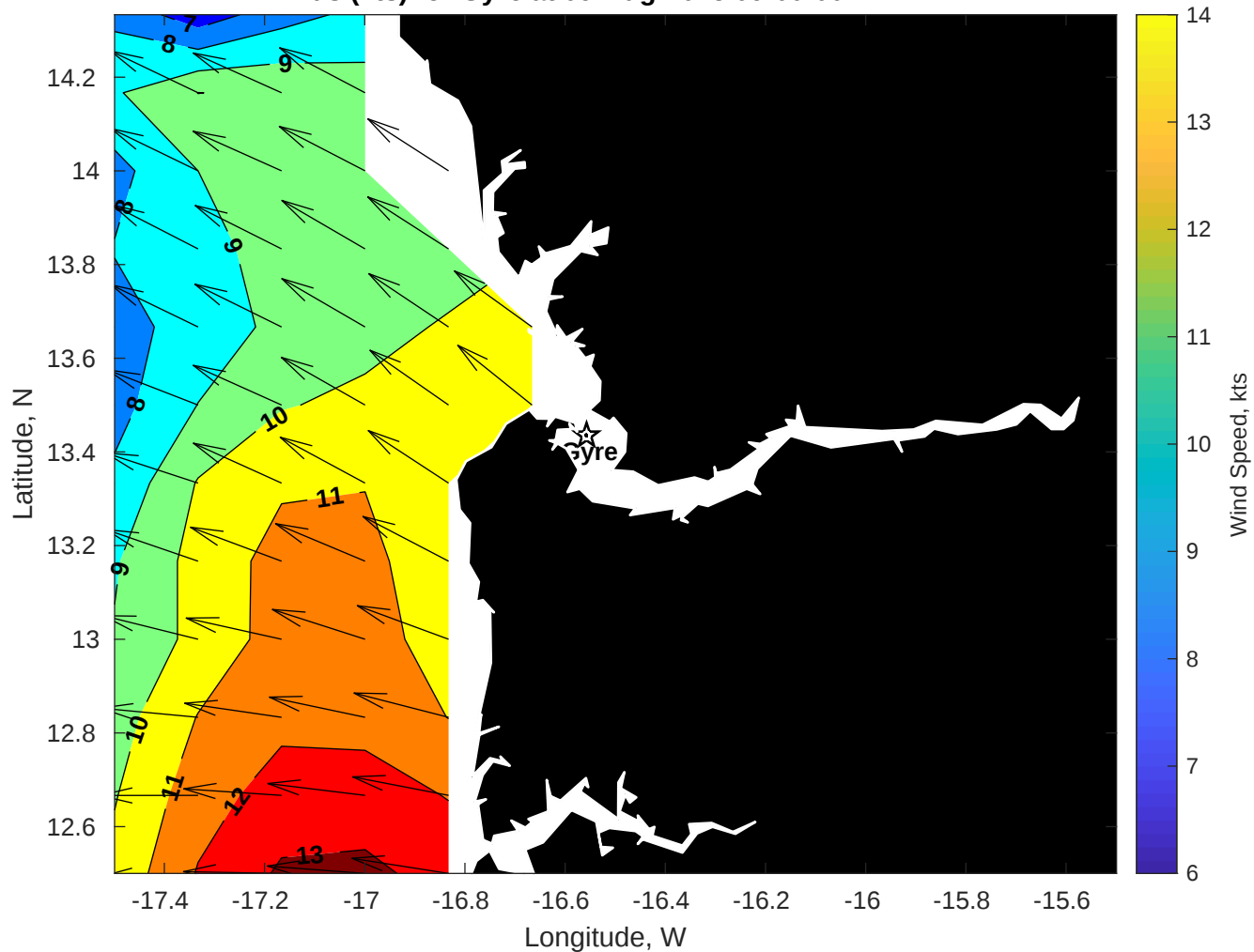
Winds (kts) for Gyre at 09-Aug-2025 09:00:00
