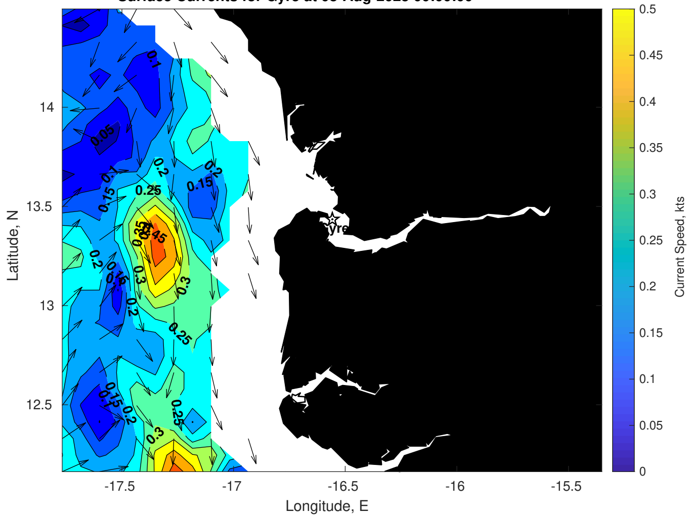
Surface Currents for Gyre at 08-Aug-2025 00:00:00
