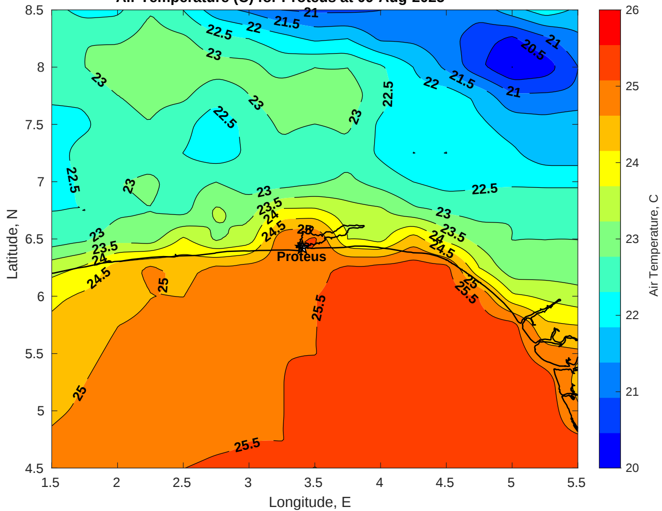
Air Temperature (C) for Proteus at 09-Aug-2025
