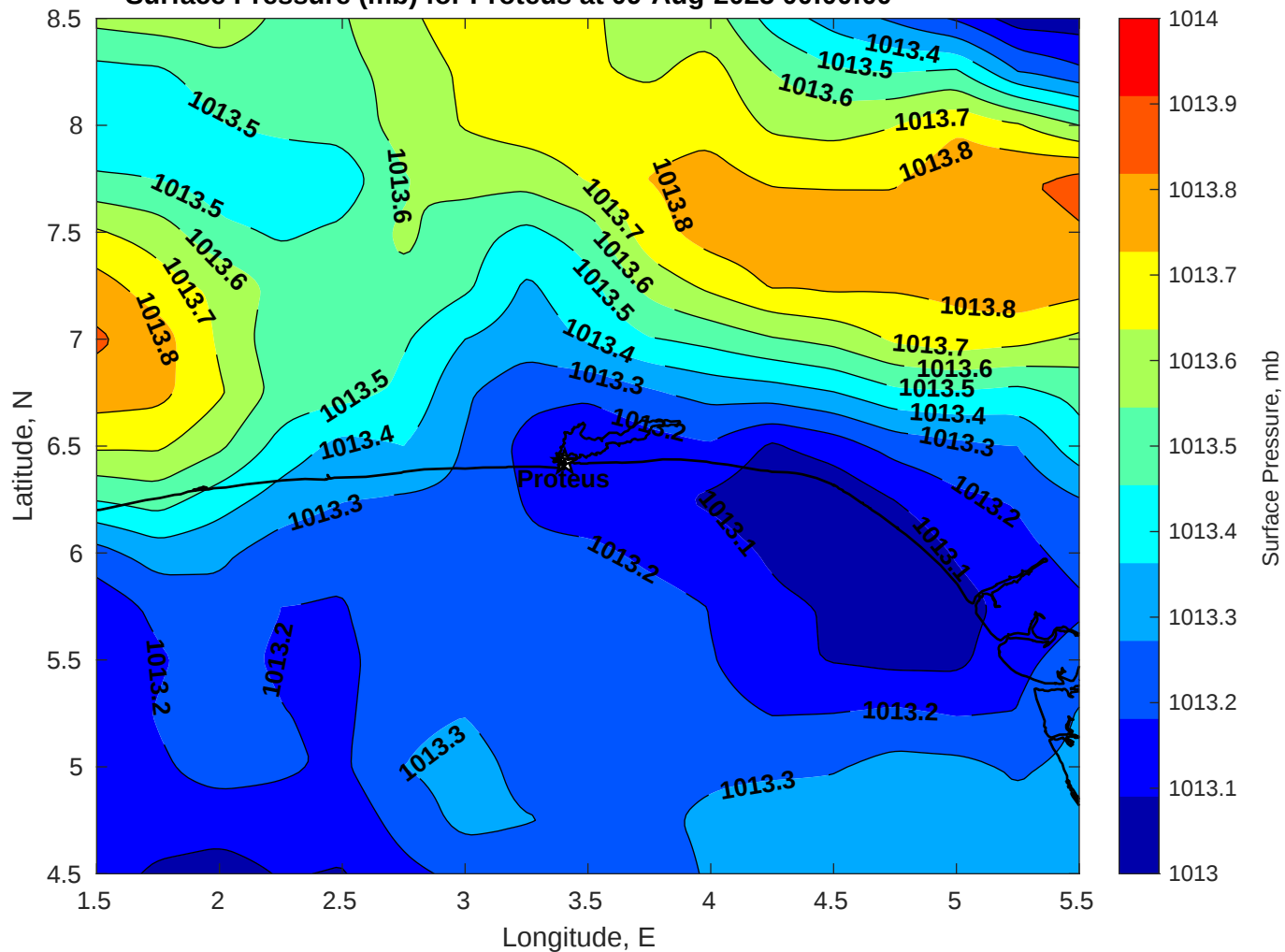
Surface Pressure (mb) for Proteus at 09-Aug-2025 00:00:00
