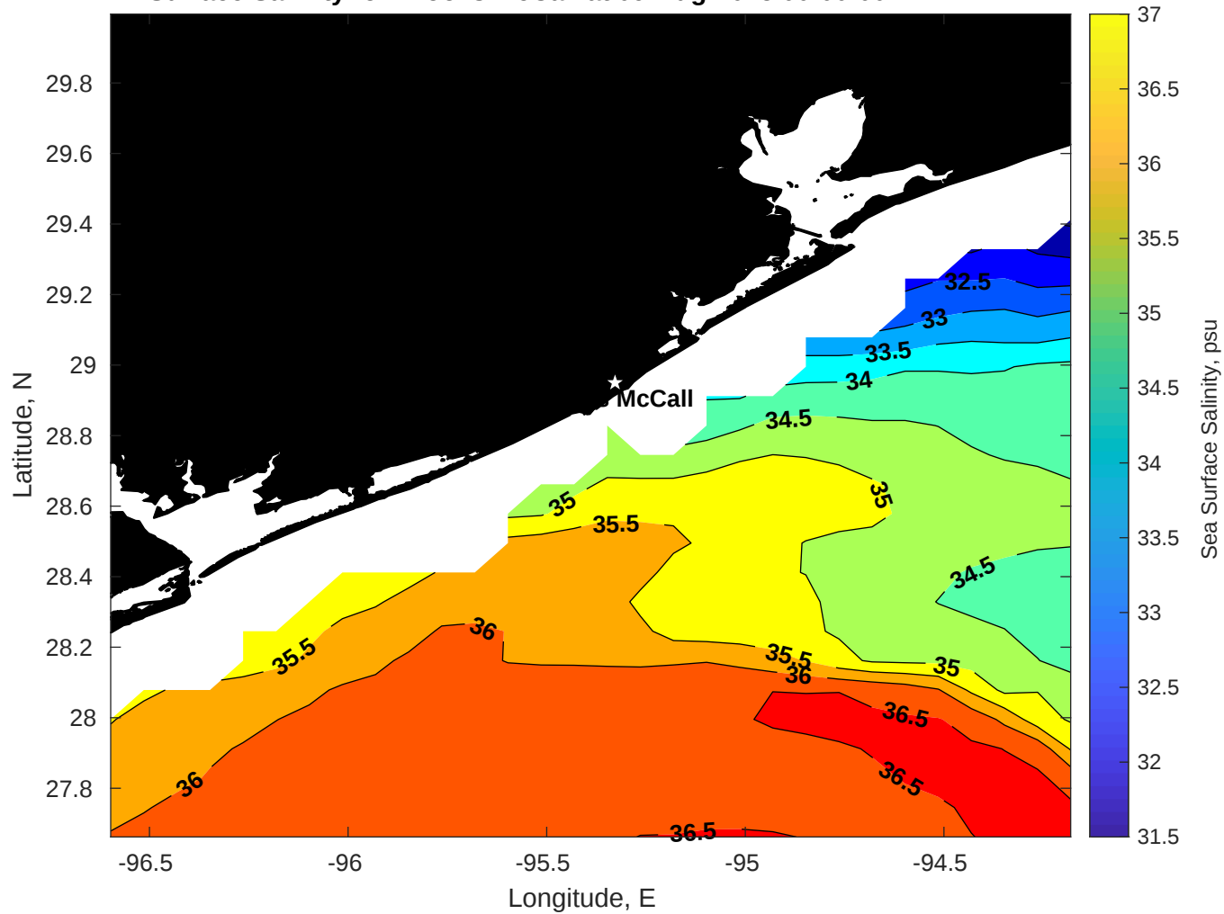
Surface Salinity for Brooks McCall at 09-Aug-2025 00:00:00
