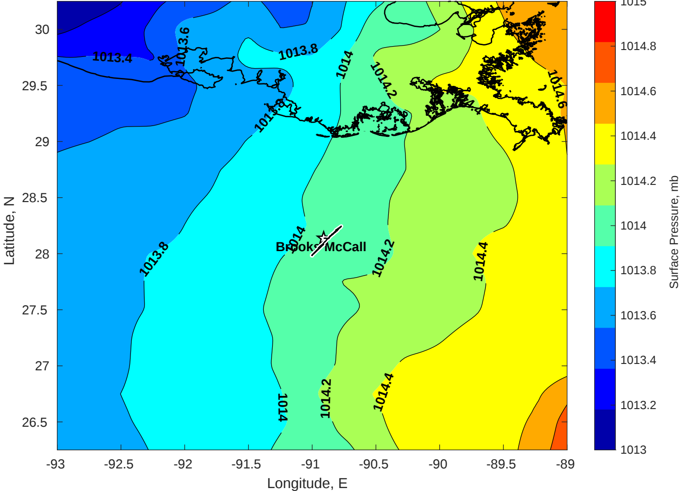
Surface Pressure (mb) for Brooks McCall at 12-Aug-2025 00:00:00
