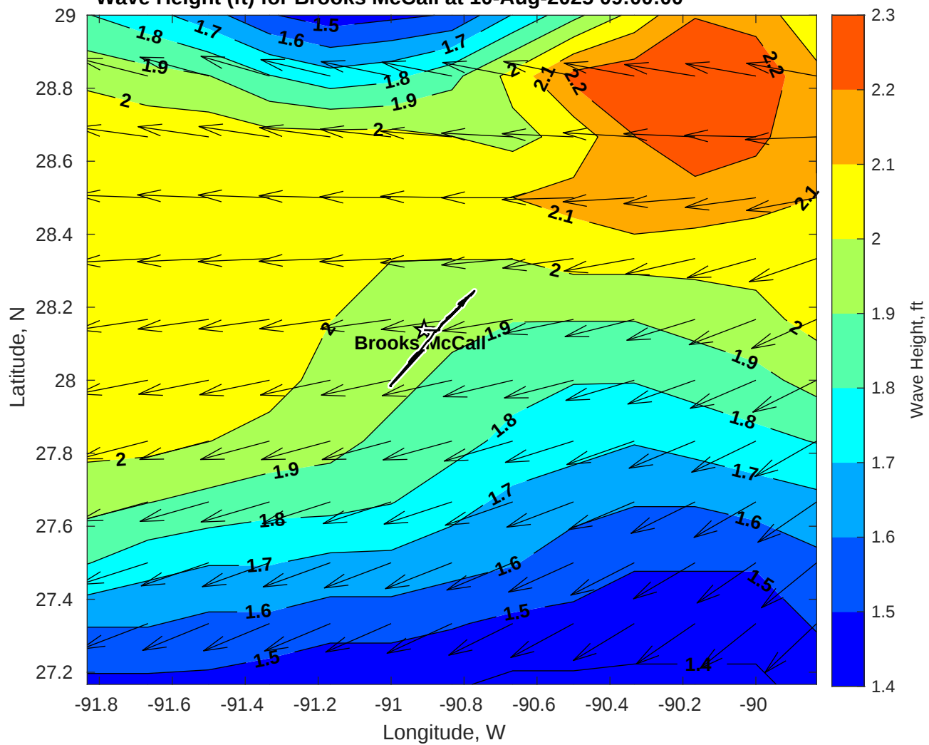
Wave Height (ft) for Brooks McCall at 10-Aug-2025 09:00:00
