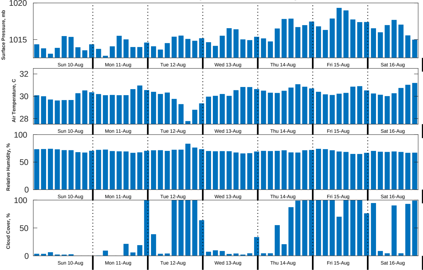
Met Forecast for Brooks McCall from 10-Aug-2025 00:00:00 to 17-Aug-2025 00:00:00
