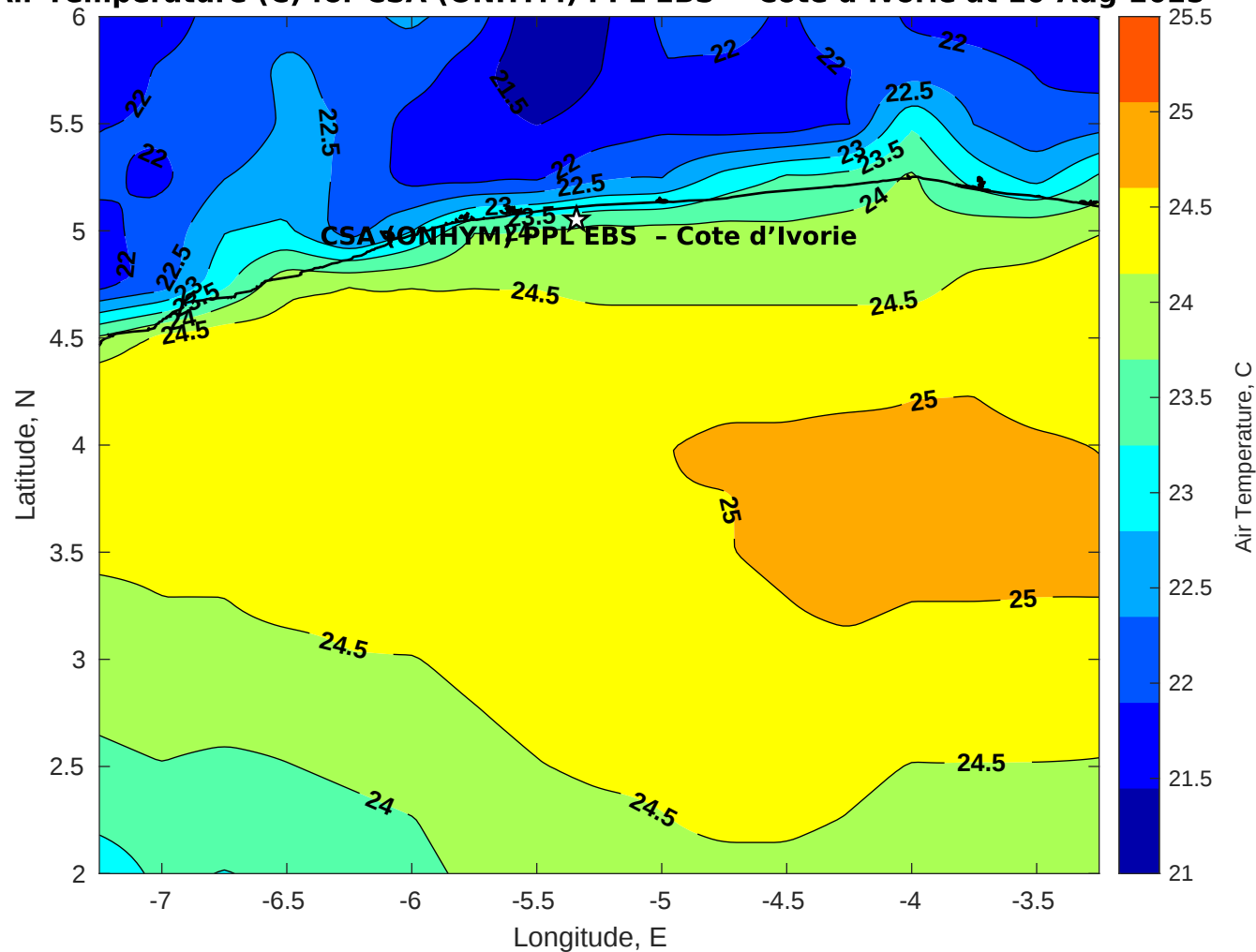
Air Temperature (C) for CSA (ONHYM) PPL EBS - Cote d'Ivoire at 10-Aug-2025
