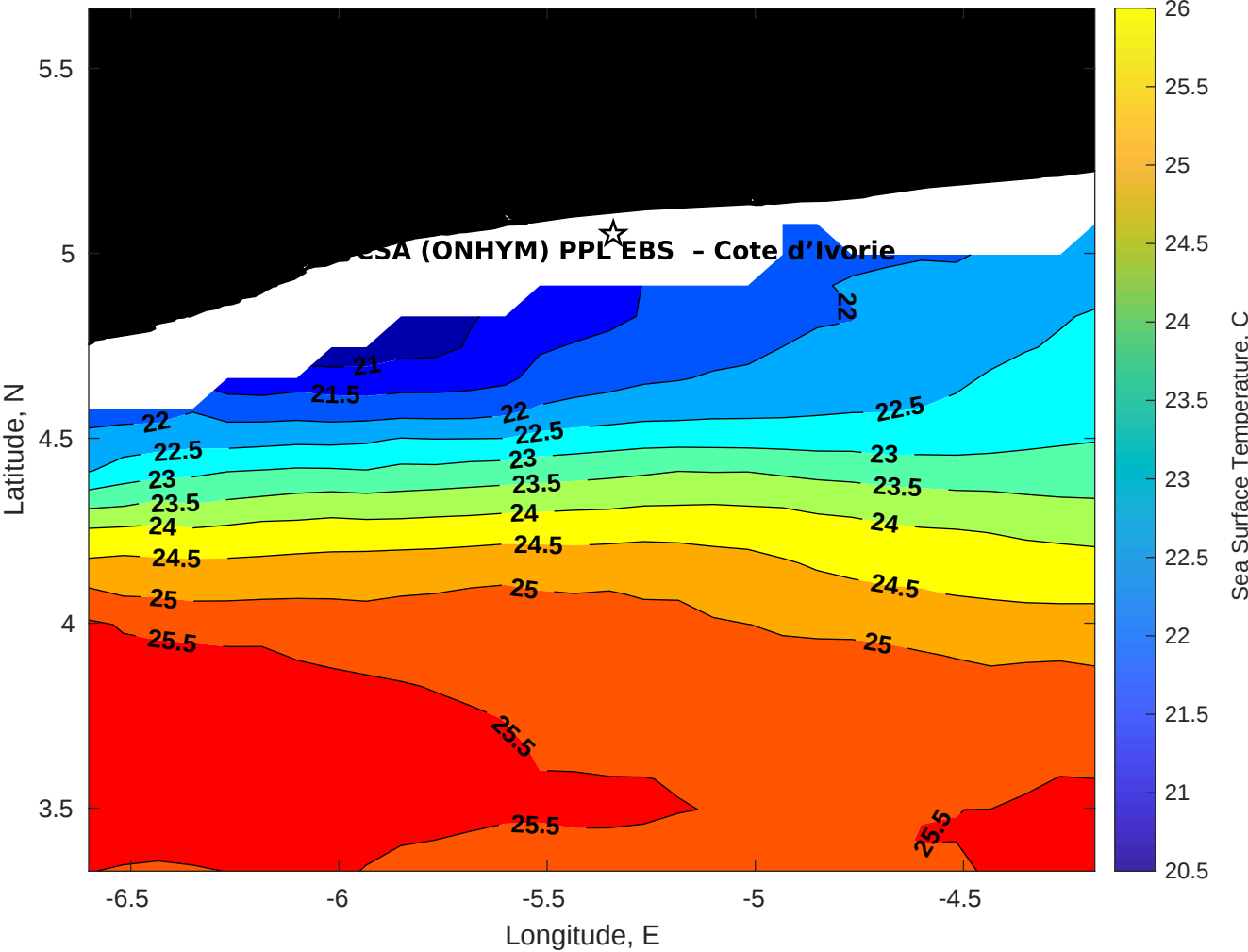
SST for CSA (ONHYM) PPL EBS - Cote d'Ivoire at 09-Aug-2025 00:00:00
